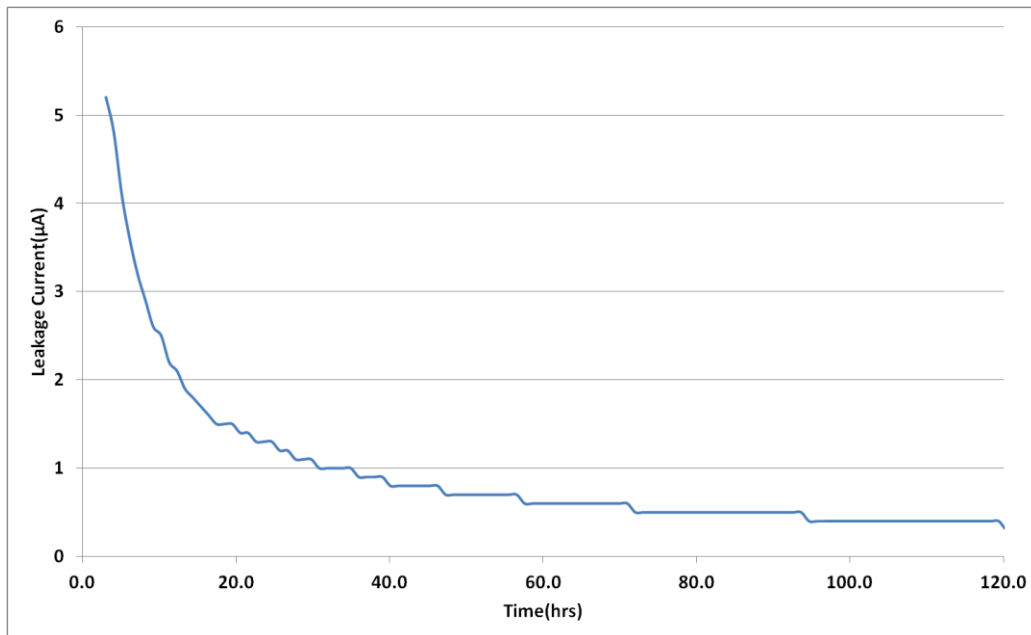
Fig 10: Leakage Current
