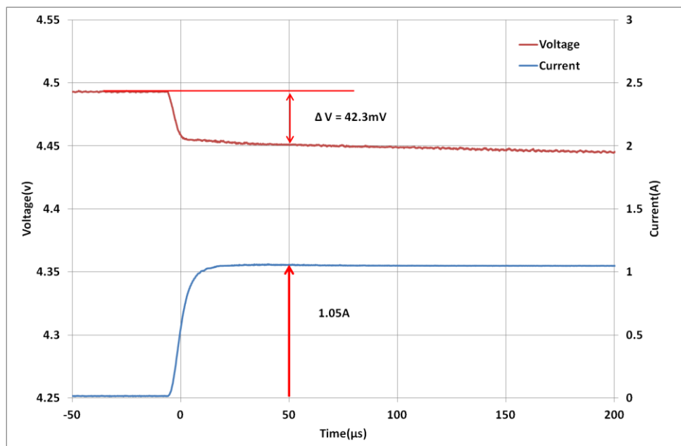
Fig 3: Measurement of ESR for a GW201
