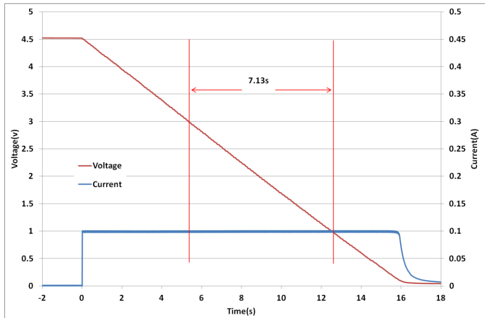
Fig 2: Measurement of DC Capacitance for a GW201
