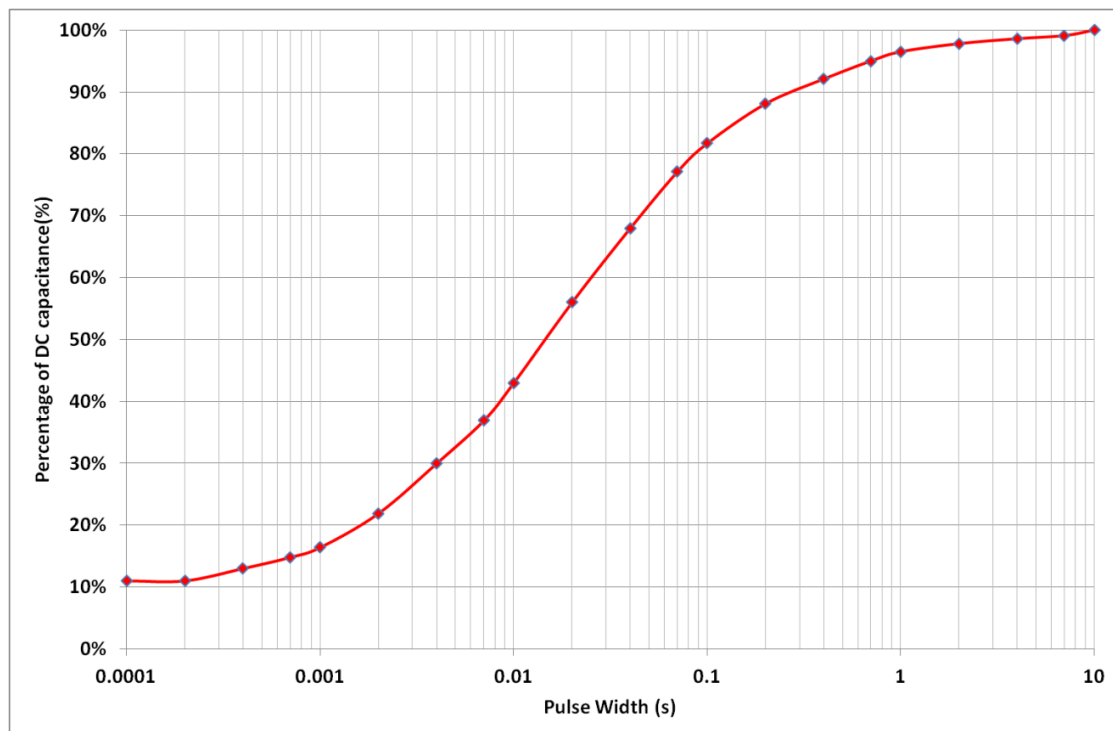
Fig 4: Effective Capacitance
