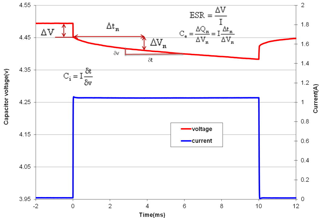
Fig 1: Effective capacitance, instantaneous capacitance and ESR for a GW201
