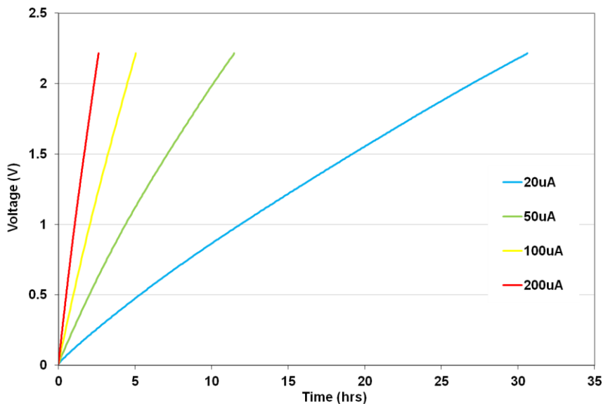
Fig 11: Charging an GW101 with low current
