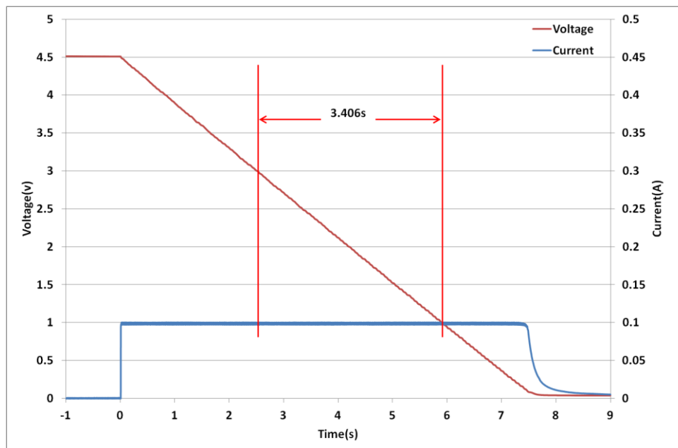
Fig 2: Measurement of DC Capacitance for a GW209
