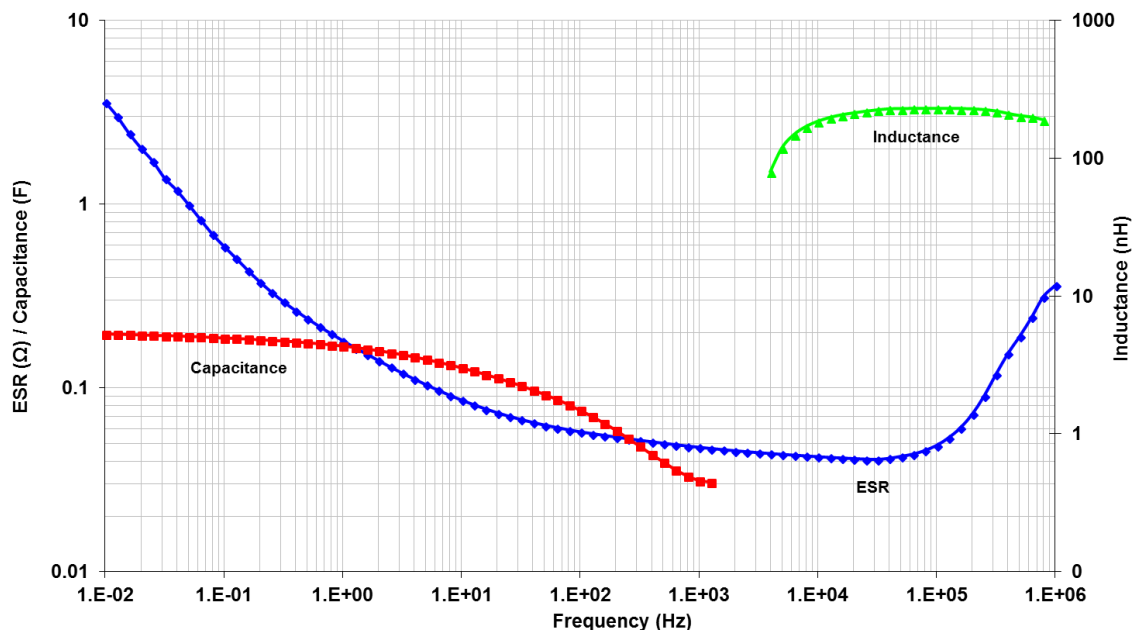
Fig 9: Frequency Response of ESR, Capacitance & Inductance
