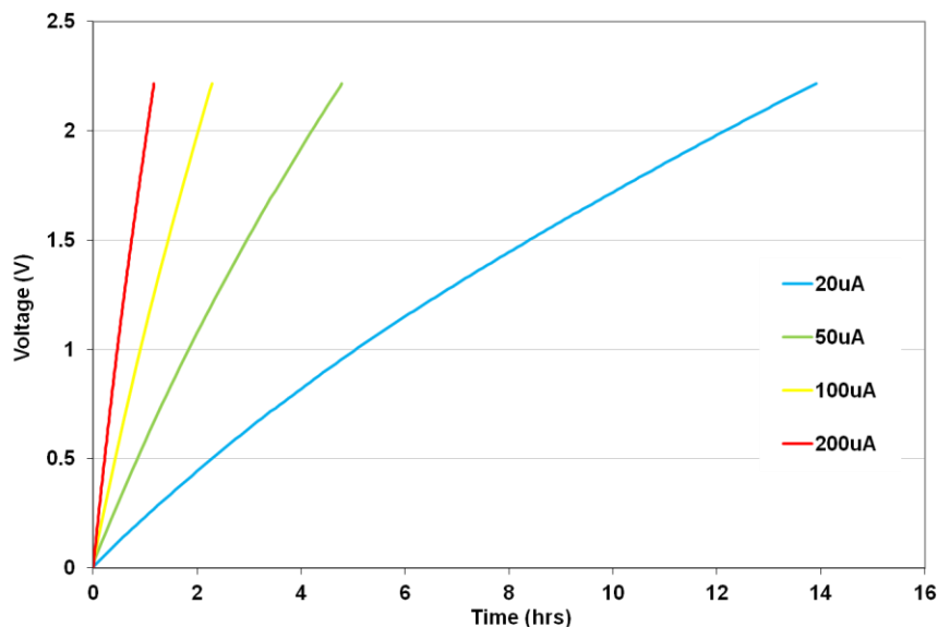
Fig 11: Charging an GW109 with low current
