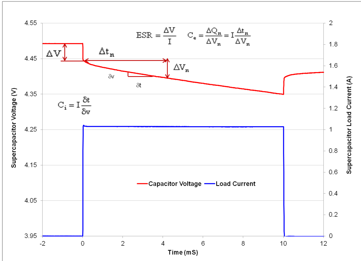
Fig 1: Effective capacitance, instantaneous capacitance and ESR for a GW209
