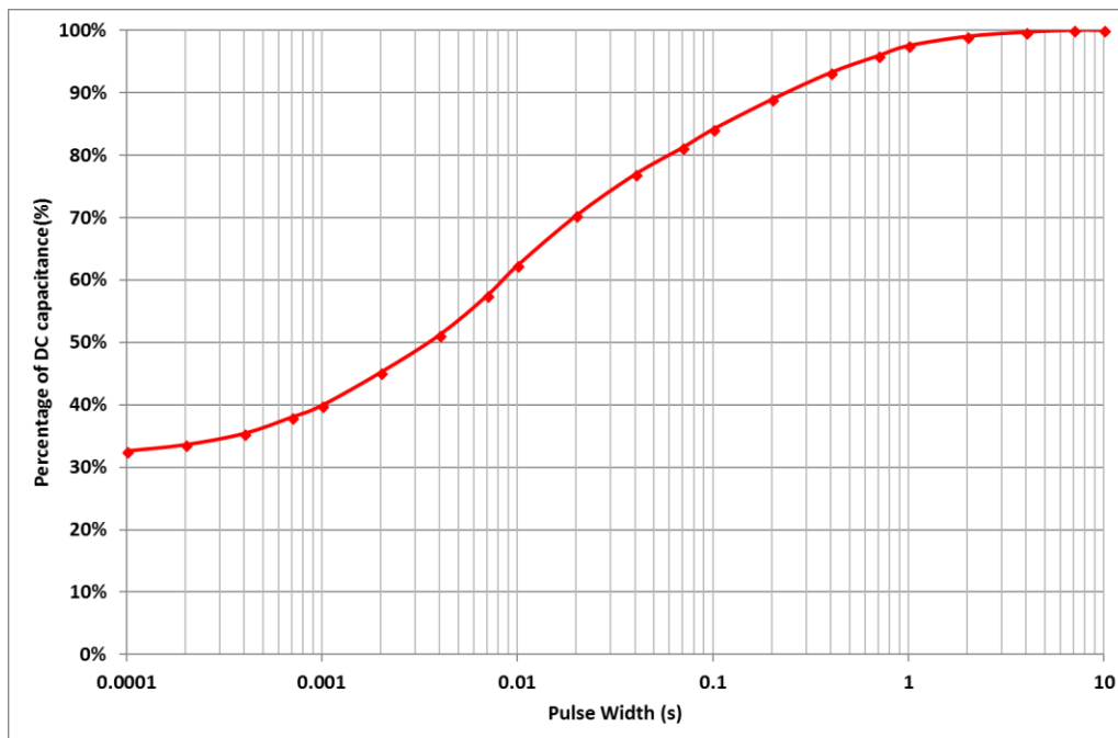
Fig 4: Effective Capacitance
