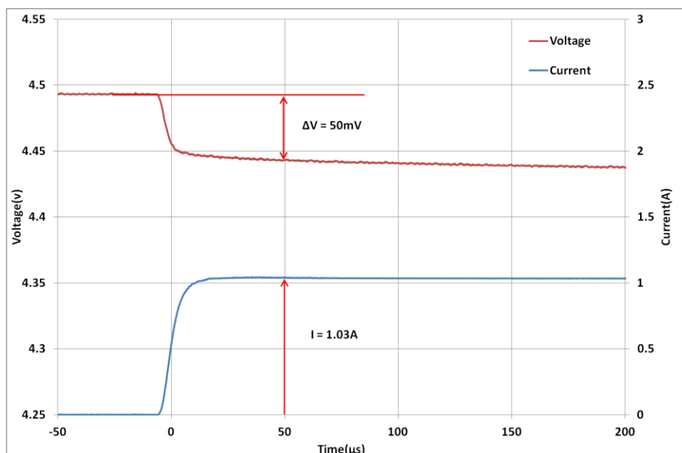
Fig 3: Measurement of ESR for a GW209
