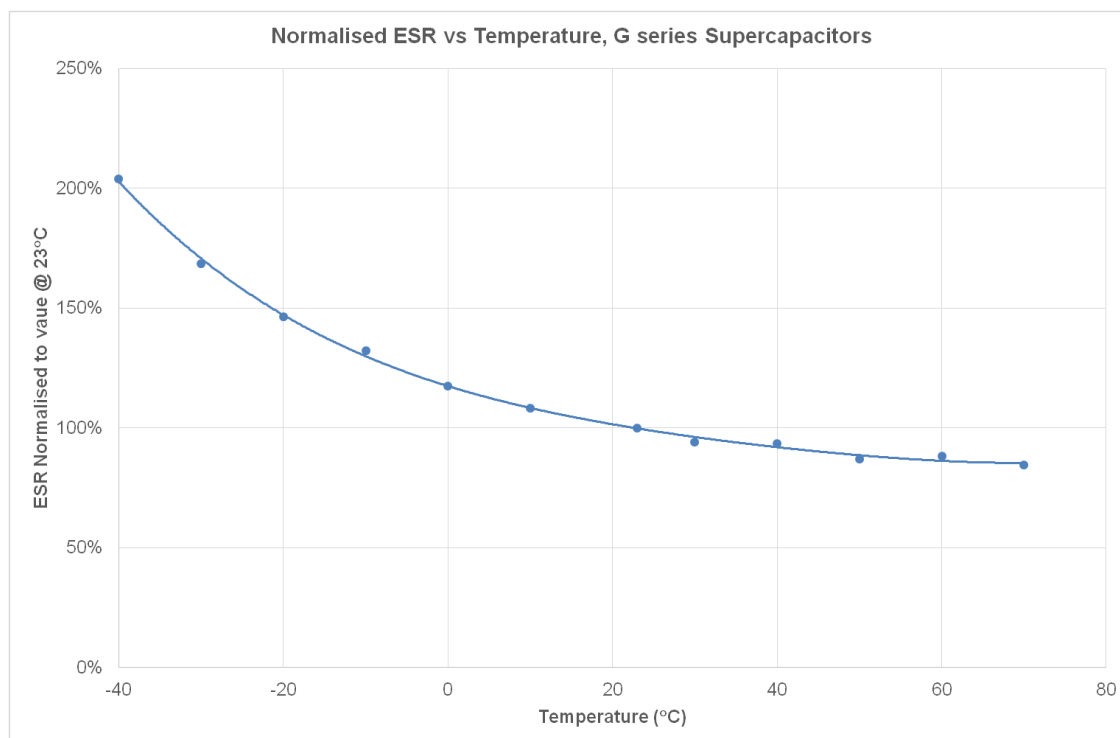
Fig 7: ESR change with temperature
