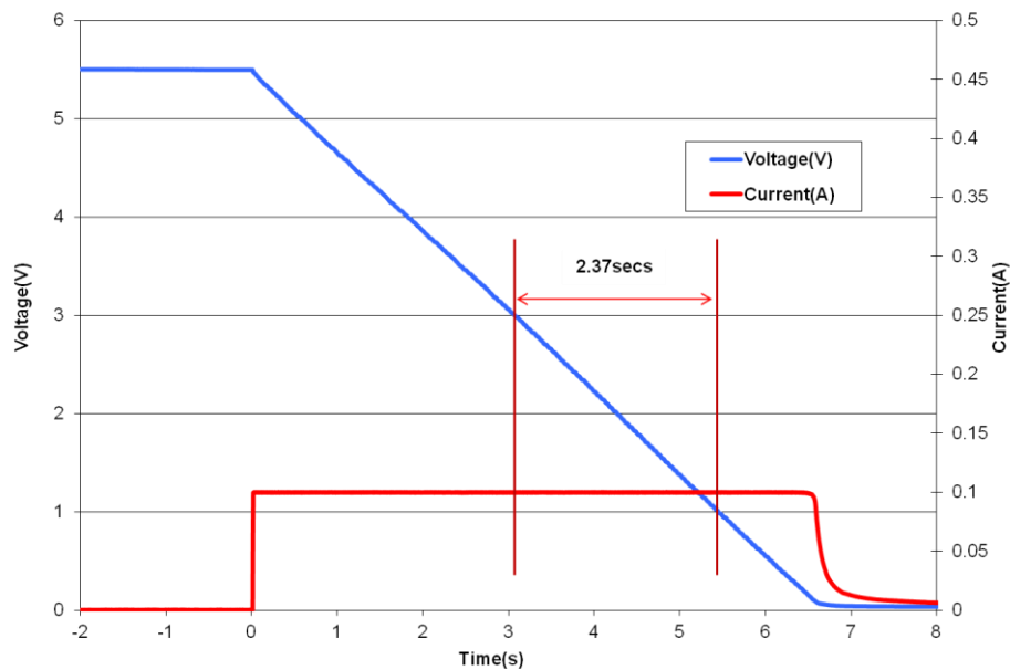
Fig 2: Measurement of DC Capacitance for an HA202
