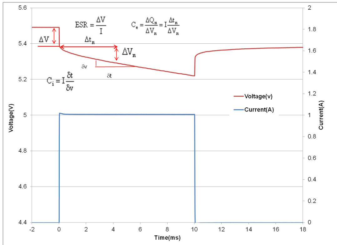
Fig 1: Effective capacitance, instantaneous capacitance and ESR for an HA202
