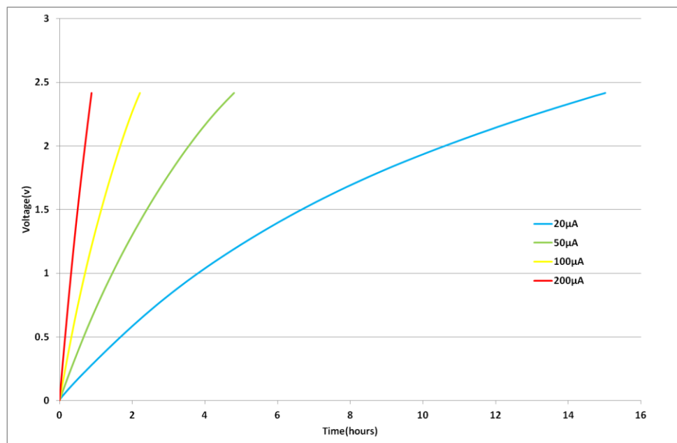
Fig 11: Charging an HA102 with low current
