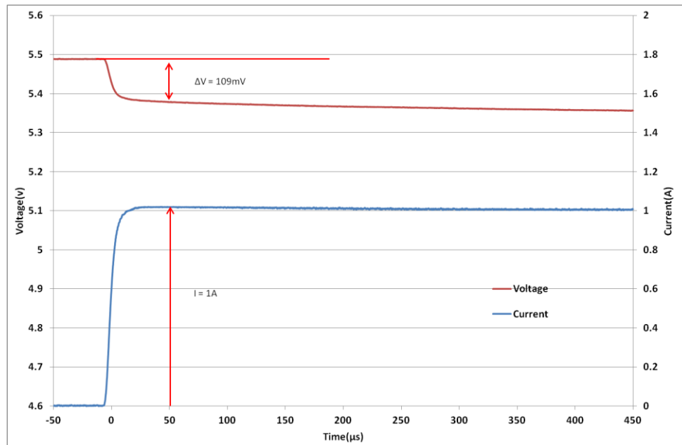
Fig 3: Measurement of ESR for an HA202
