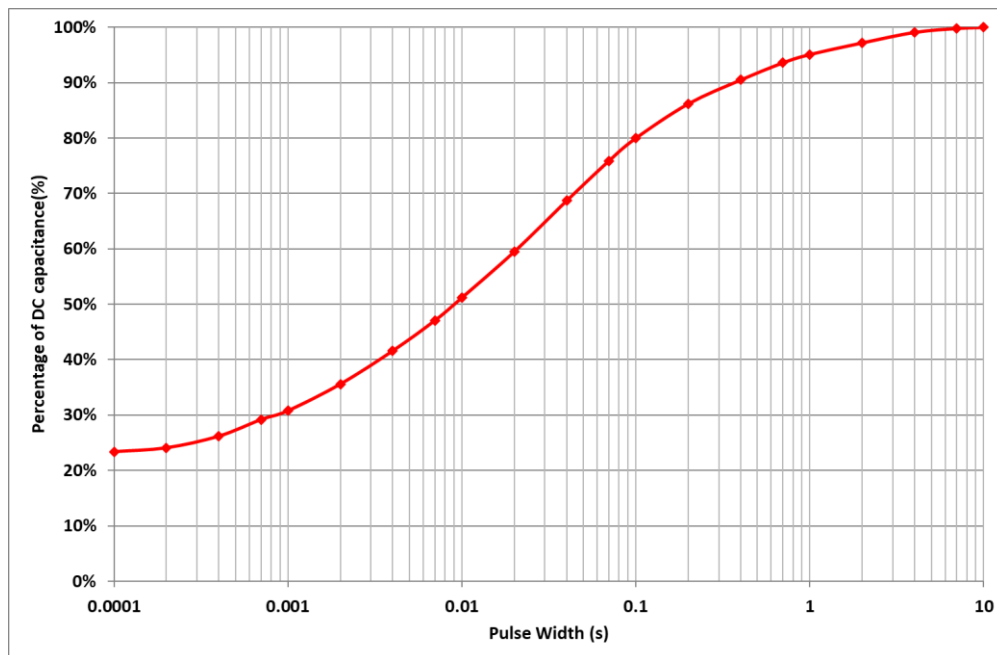
Figure 4: Effective Capacitance
