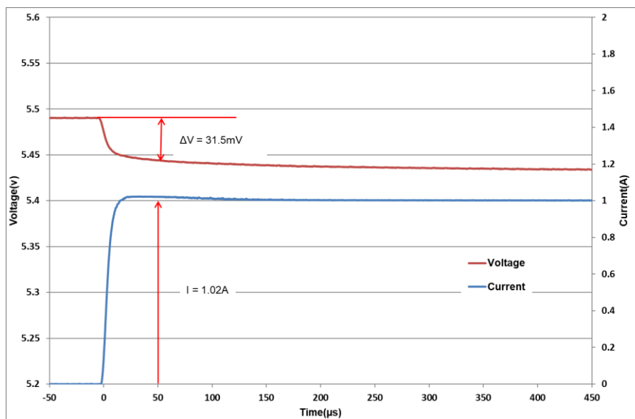
Fig 3: Measurement of ESR for a DMF4B5R5G105M3DTA0
