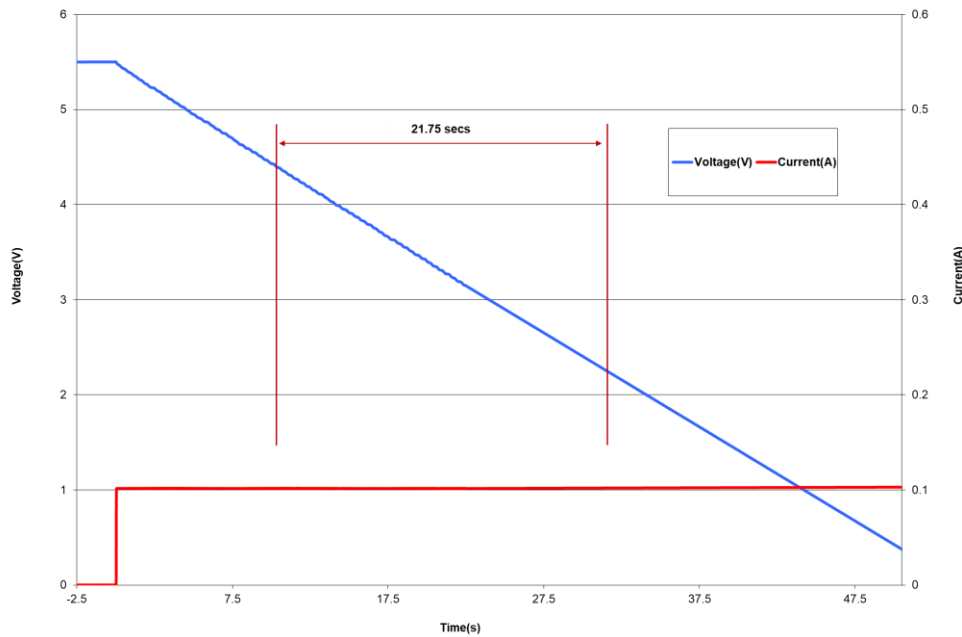
Fig 2: Measurement of DC Capacitance for a DMF4B5R5G105M3DTA0
