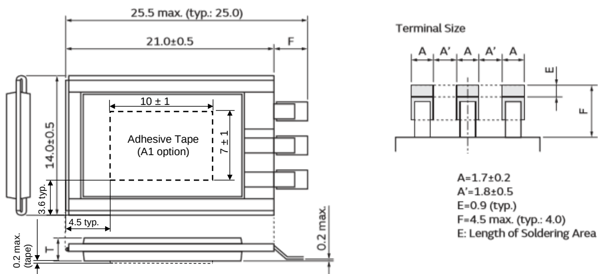
Mechanical drawing for DMF3Z5R5H474M3DTA0
