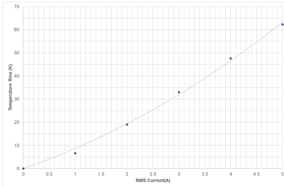
Fig 12: Temperature rise in DMT334R2S474M3DTA0 with RMS current
