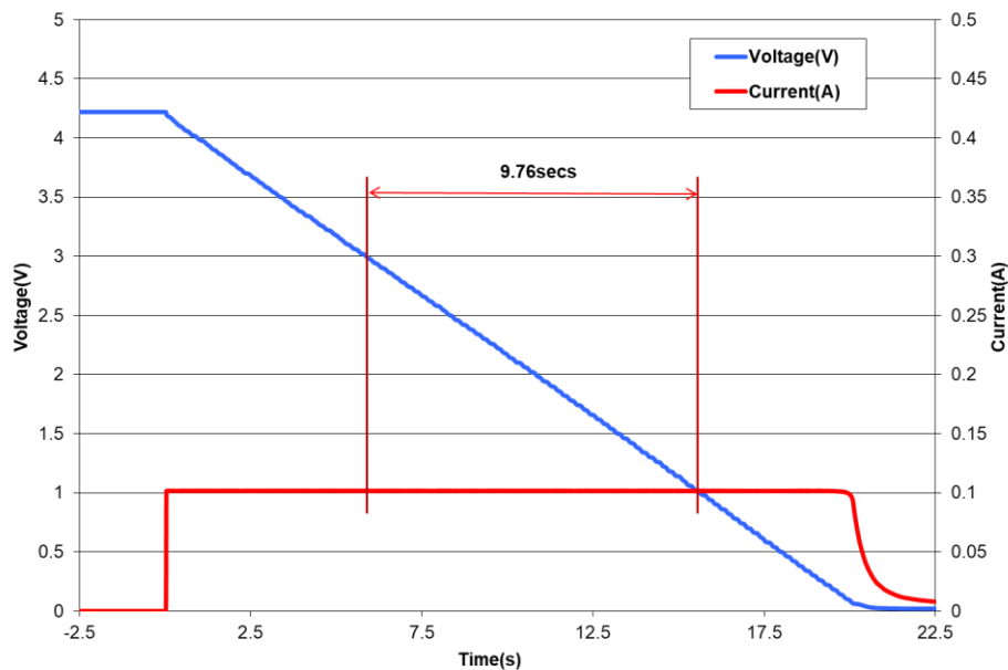
Fig 2: Measurement of DC Capacitance for DMT334R2S474M3DTA0
