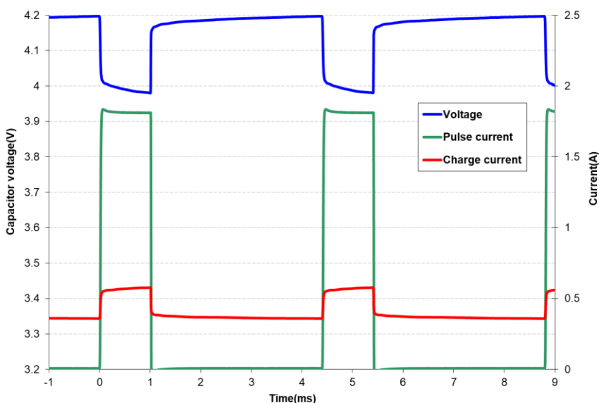
Fig 5: DMT334R2S474M3DTA0 Pulse Response with GPRS Class 10 Pulse Train
