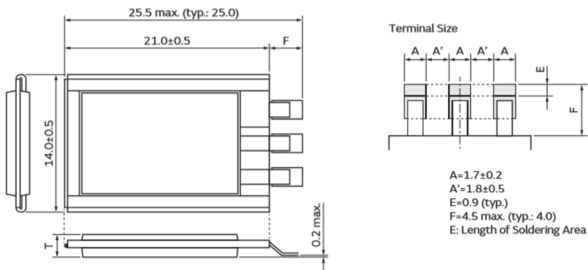
Mechanical drawing for DMT334R2S474 M3DTA0
