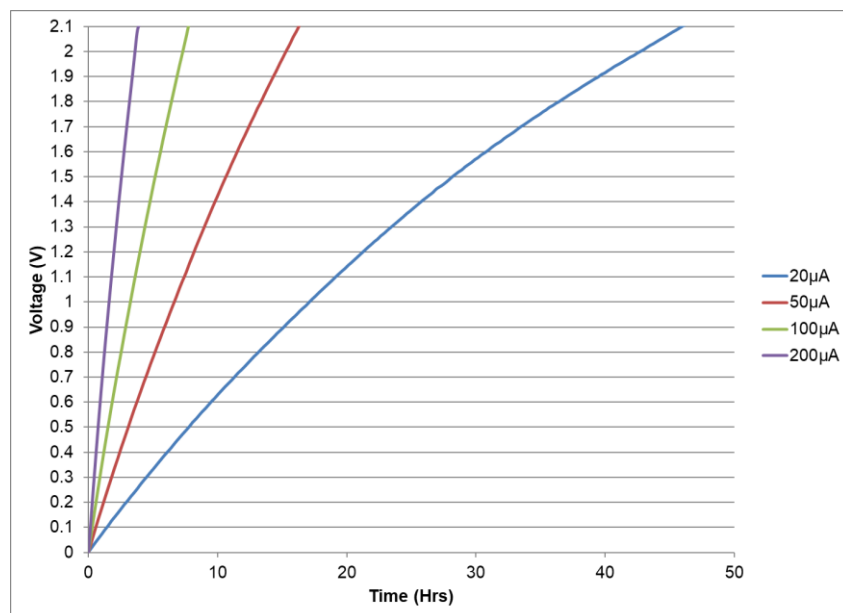
Fig 11: Charging a single cell of DMT334R2S474M3DTA0 (single cell: 940mF) with low current
