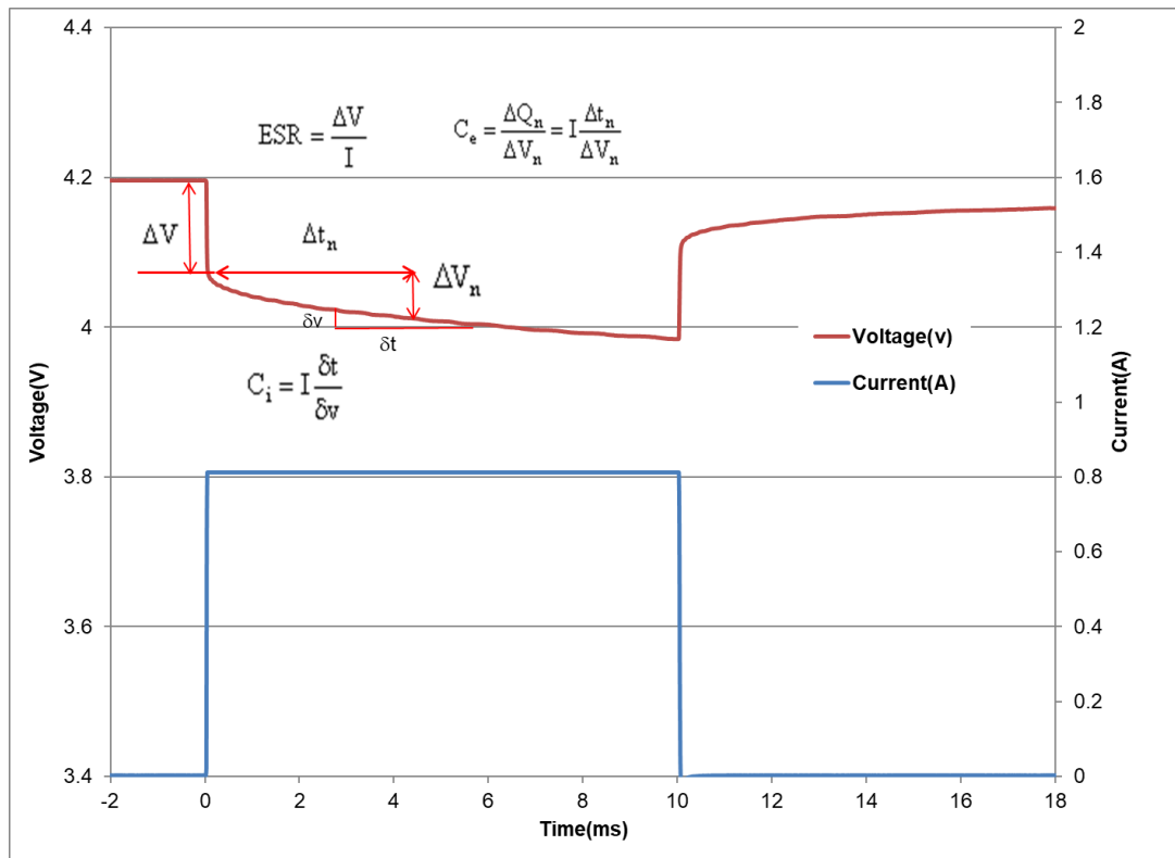
Fig 1: Effective capacitance, instantaneous capacitance and ESR for DMT334R2S474M3DTA0
