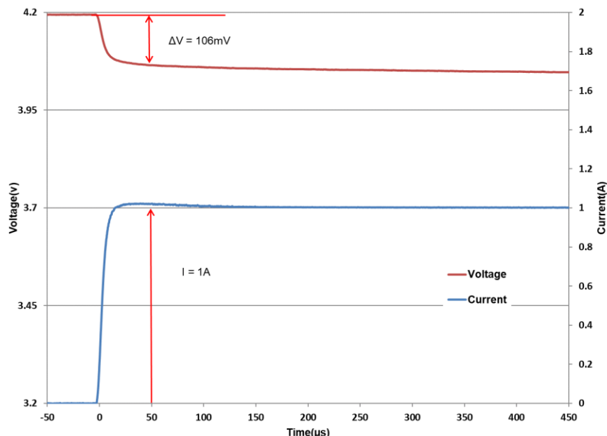
Fig 3: Measurement of ESR for a DMT334R2S474M3DTA0
