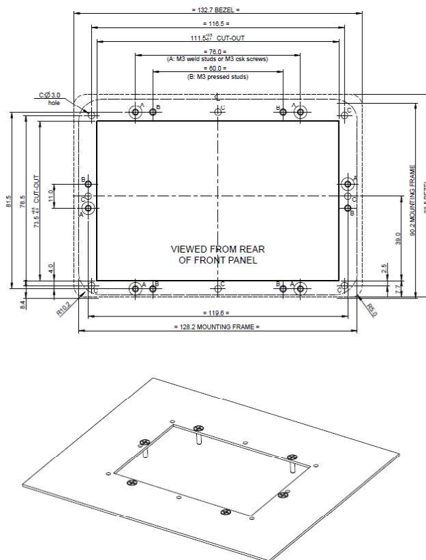
Figure 25 - IDM2040-43A Panel Mount Dimensions
