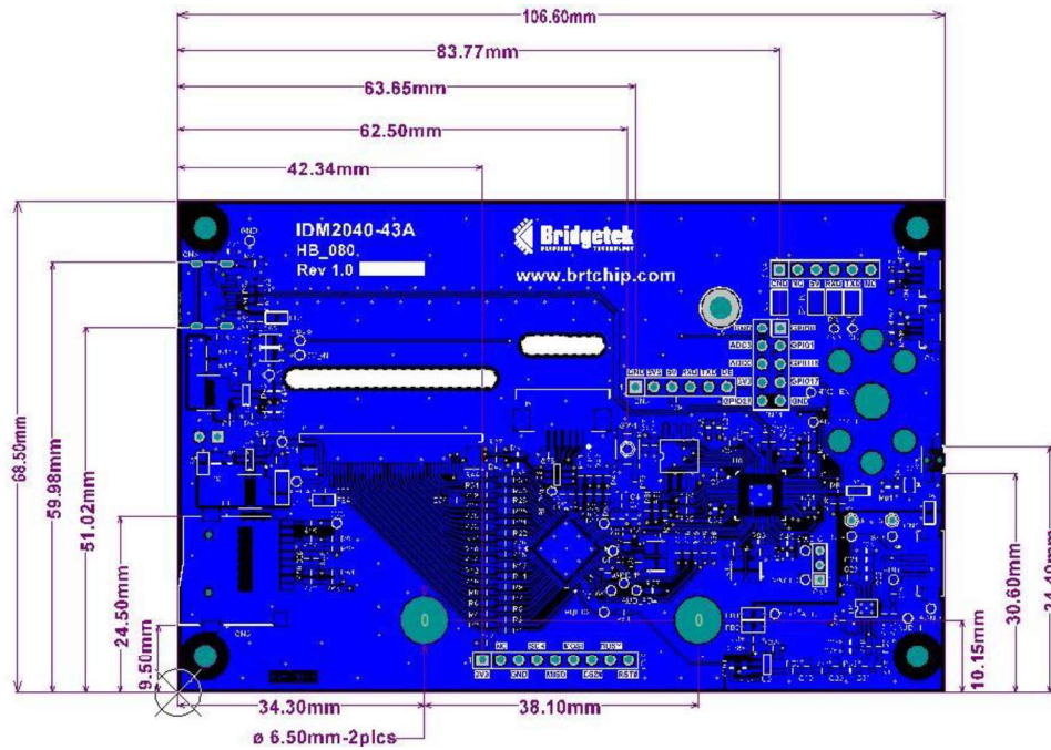
Figure 16 – IDM2040-43A PCBA Dimensions (Top View)
