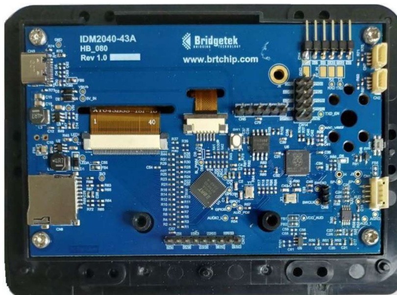
Figure 2 - IDM2040-43A Module - Back View
