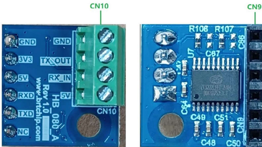
Figure 7 – Connectors on IDM-RS232
