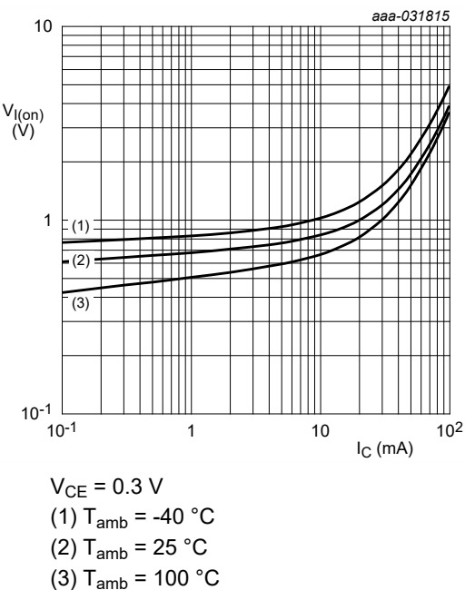
Fig. 6. NHDTC123JT-Q: On-state input voltage as a function of collector current; typical values
