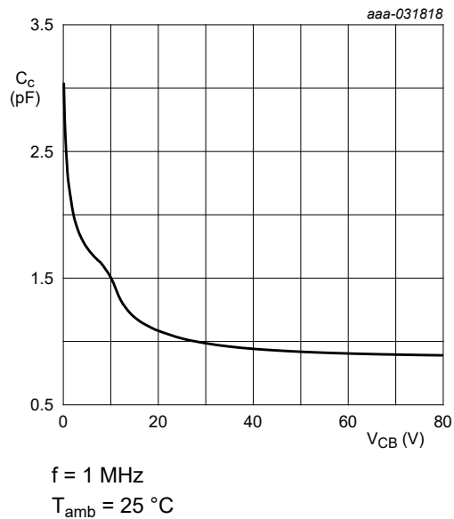
Fig. 9. NHDTC123JT-Q: Collector capacitance as a function of collector-base voltage; typical values
