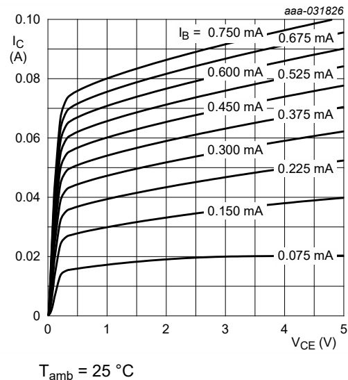
Fig. 17. NHDTC114YT-Q: Collector current as a function of collector-emitter voltage; typical values
