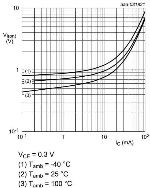
Fig. 12. NHDTC143ZT-Q: On-state input voltage as a function of collector current; typical values
