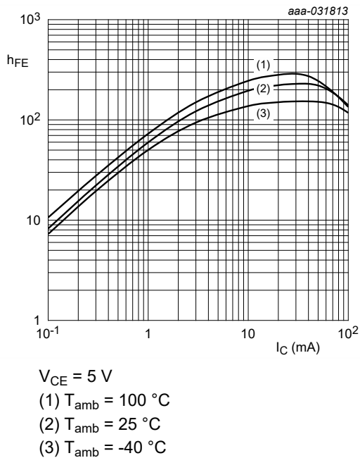
Fig. 4. NHDTC123JT-Q: DC current gain as a function of collector current; typical values
