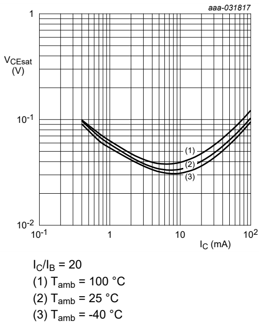
Fig. 8. NHDTC123JT-Q: Collector-emitter saturation voltage as a function of collector current; typical values
