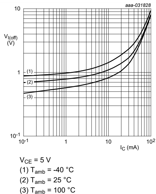
Fig. 19. NHDTC114YT-Q: Off-state input voltage as a function of collector current; typical values
