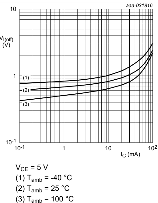
Fig. 7. NHDTC123JT-Q: Off-state input voltage as a function of collector current; typical values
