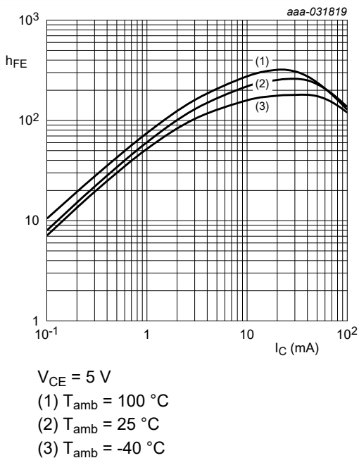
Fig. 10. NHDTC143ZT-Q: DC current gain as a function of collector current; typical values
