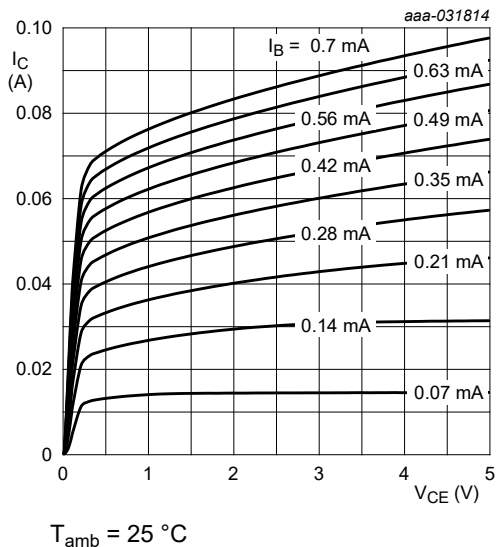
Fig. 5. NHDTC123JT-Q: Collector current as a function of collector-emitter voltage; typical values
