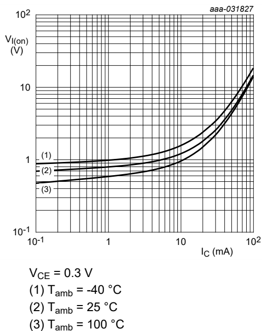
Fig. 18. NHDTC114YT-Q: On-state input voltage as a function of collector current; typical values
