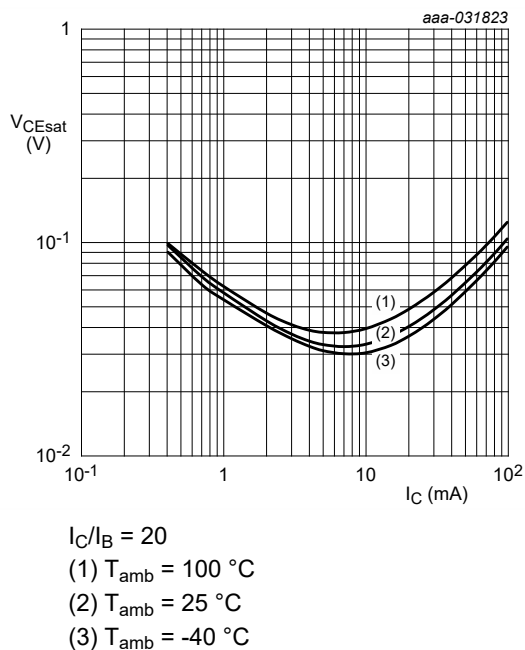
Fig. 14. NHDTC143ZT-Q: Collector-emitter saturation voltage as a function of collector current; typical values
