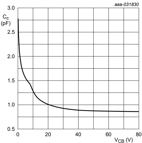
Fig. 21. NHDTC114YT-Q: Collector capacitance as a function of collector-base voltage; typical values
