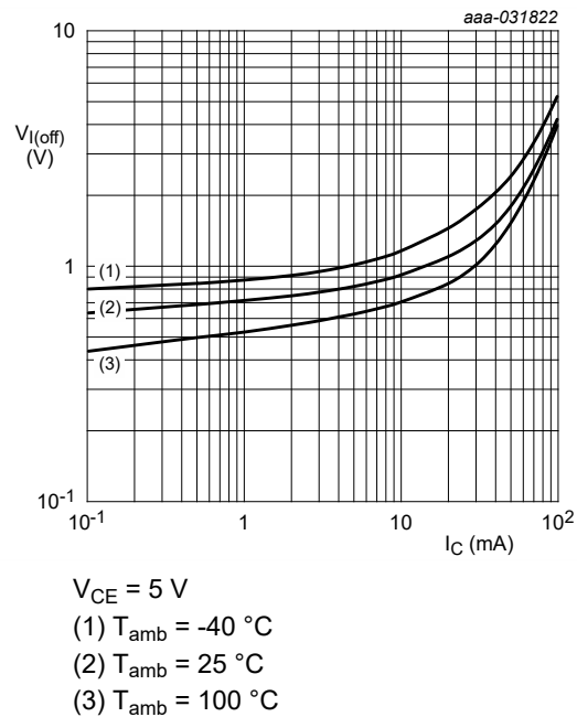
Fig. 13. NHDTC143ZT-Q: Off-state input voltage as a function of collector current; typical values
