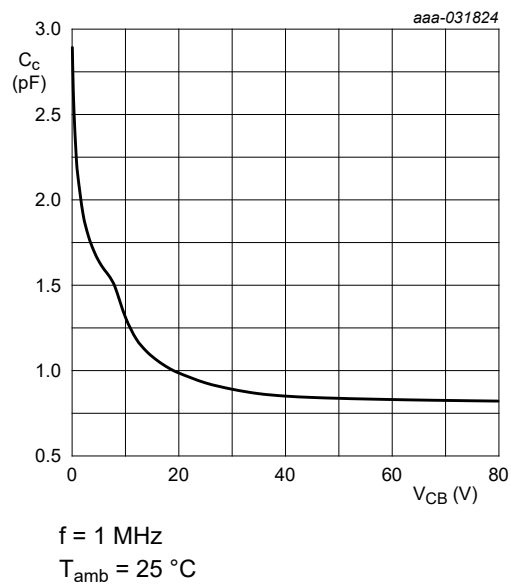
Fig. 15. NHDTC143ZT-Q: Collector capacitance as a function of collector-base voltage; typical values
