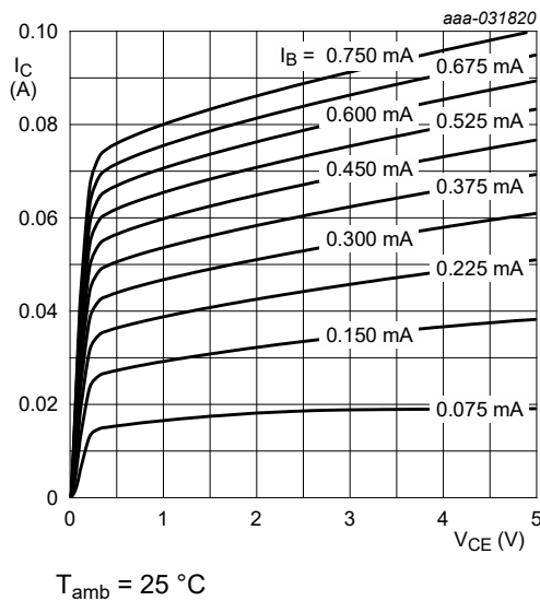
Fig. 11. NHDTC143ZT-Q: Collector current as a function of collector-emitter voltage; typical values
