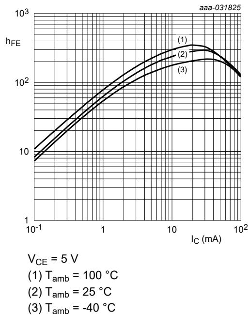
Fig. 16. NHDTC114YT-Q: DC current gain as a function of collector current; typical values
