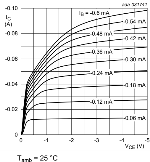
Fig. 5. NHDTA123JT-Q: Collector current as a function of collector-emitter voltage; typical values
