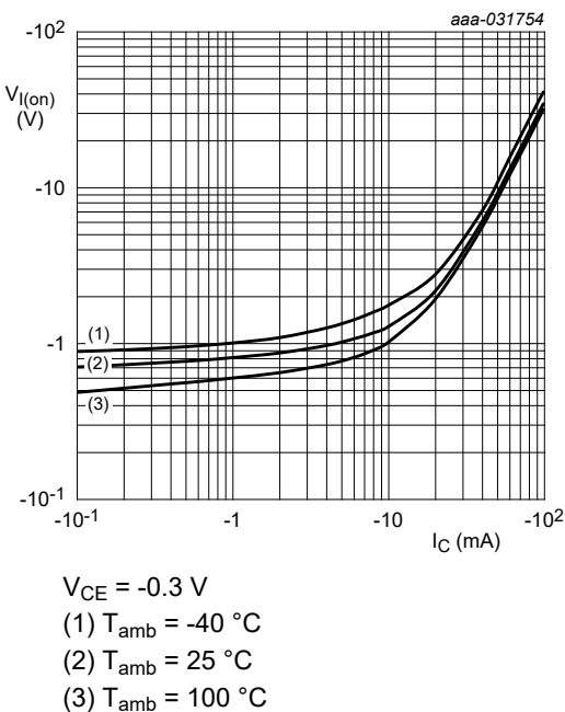
Fig. 18. NHDTA114YT-Q: On-state input voltage as a function of collector current; typical values
