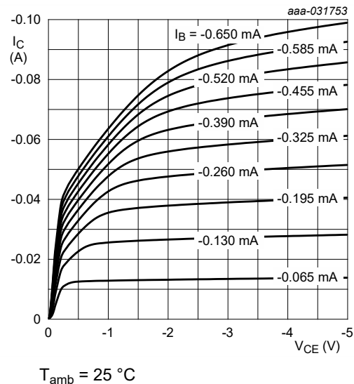
Fig. 17. NHDTA114YT-Q: Collector current as a function of collector-emitter voltage; typical values
