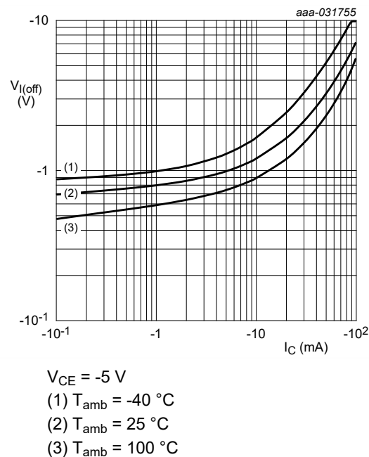
Fig. 19. NHDTA114YT-Q: Off-state input voltage as a function of collector current; typical values
