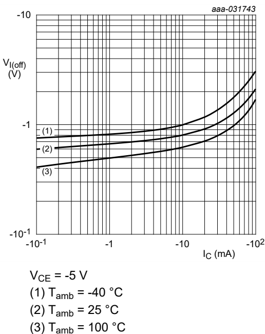
Fig. 7. NHDTA123JT-Q: Off-state input voltage as a function of collector current; typical values
