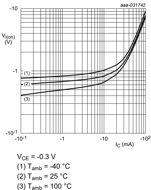
Fig. 6. NHDTA123JT-Q: On-state input voltage as a function of collector current; typical values
