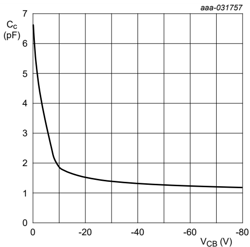
Fig. 21. NHDTA114YT-Q: Collector capacitance as a function of collector-base voltage; typical values
