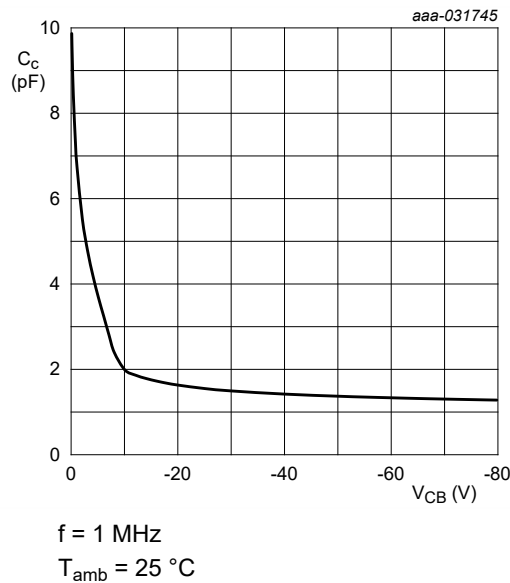
Fig. 9. NHDTA123JT-Q: Collector capacitance as a function of collector-base voltage; typical values
