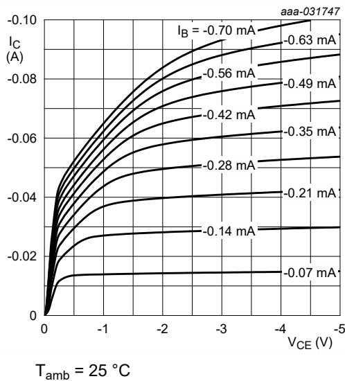
Fig. 11. NHDTA143ZT-Q: Collector current as a function of collector-emitter voltage; typical values
