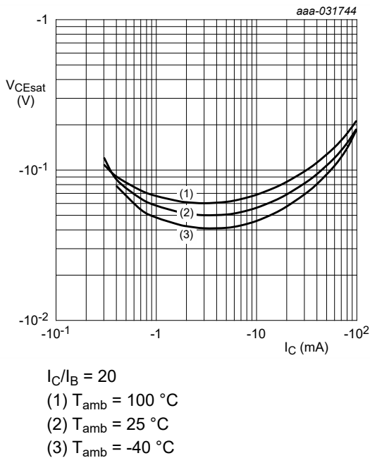
Fig. 8. NHDTA123JT-Q: Collector-emitter saturation voltage as a function of collector current; typical values
