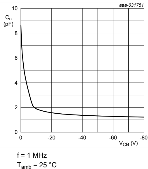
Fig. 15. NHDTA143ZT-Q: Collector capacitance as a function of collector-base voltage; typical values
