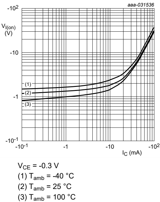
Fig. 6. NHDTA114ET-Q: On-state input voltage as a function of collector current; typical values
