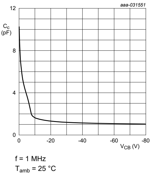
Fig. 21. NHDTA144ET-Q: Collector capacitance as a function of collector-base voltage; typical values of built-in transistor
