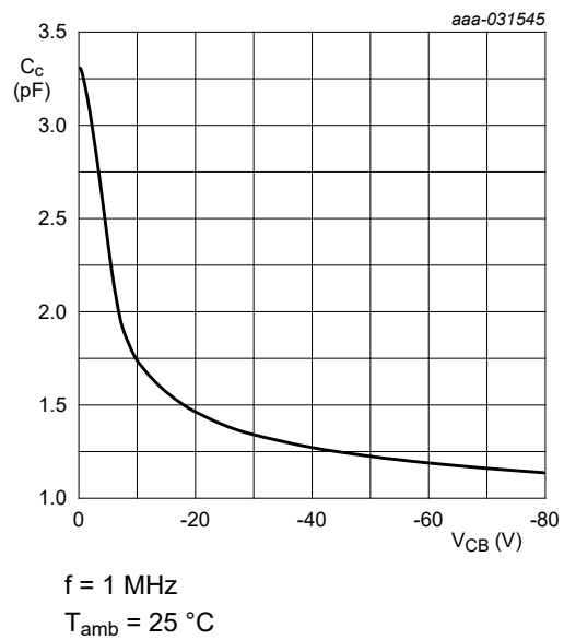
Fig. 15. NHDTA124ET-Q: Collector capacitance as a function of collector-base voltage; typical values
