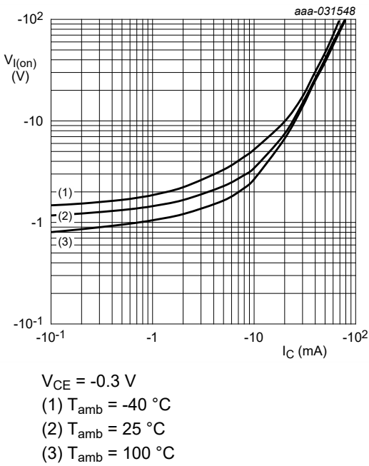
Fig. 18. NHDTA144ET-Q: On-state input voltage as a function of collector current; typical values
