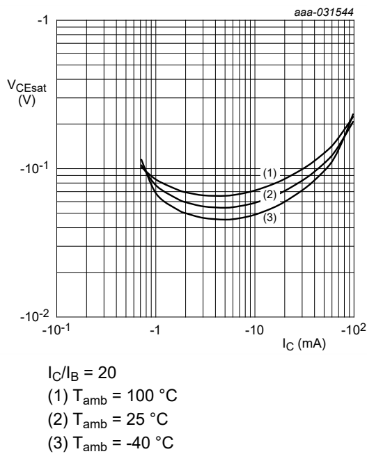
Fig. 14. NHDTA124ET-Q: Collector-emitter saturation voltage as a function of collector current; typical values
