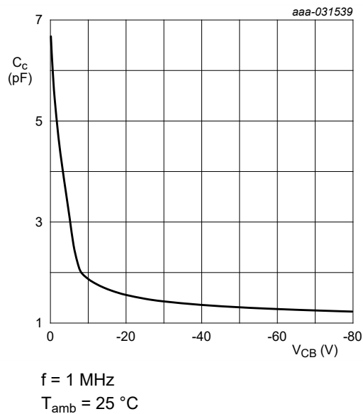
Fig. 9. NHDTA114ET-Q: Collector capacitance as a function of collector-base voltage; typical values
