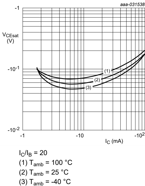
Fig. 8. NHDTA114ET-Q: Collector-emitter saturation voltage as a function of collector current; typical values
