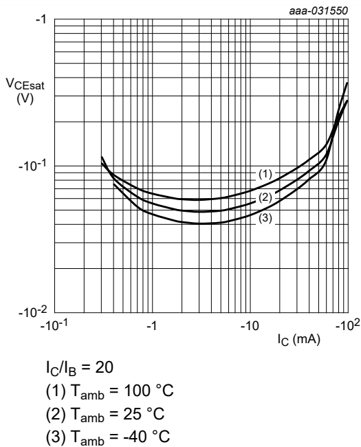
Fig. 20. NHDTA144ET-Q: Collector-emitter saturation voltage as a function of collector current; typical values
