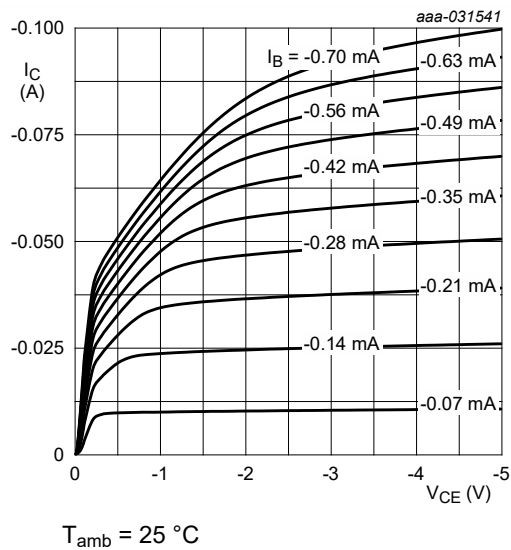
Fig. 11. NHDTA124ET-Q: Collector current as a function of collector-emitter voltage; typical values
