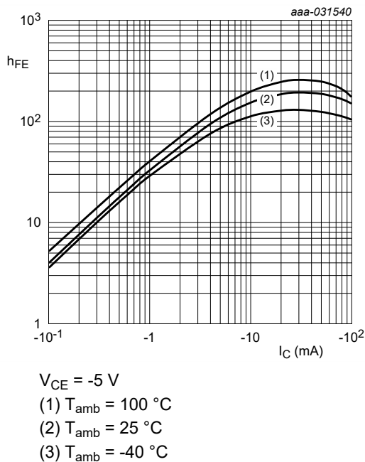
Fig. 10. NHDTA124ET-Q: DC current gain as a function of collector current; typical values
