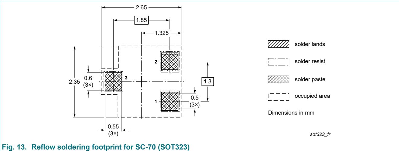
Fig. 13. Reflow soldering footprint for SC-70 (SOT323)
