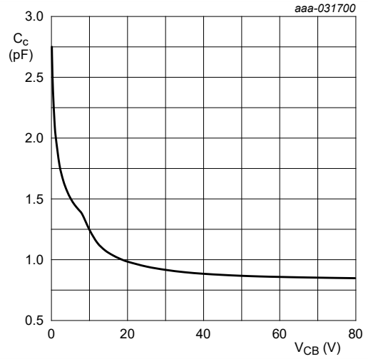
Fig. 8. NHUMD3-Q, TR1 (NPN): Collector capacitance as a function of collector-base voltage; typical values
