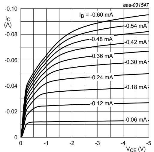
Fig. 34. NHUMD12-Q, TR2 (PNP): Collector current as a function of collector-emitter voltage; typical values
