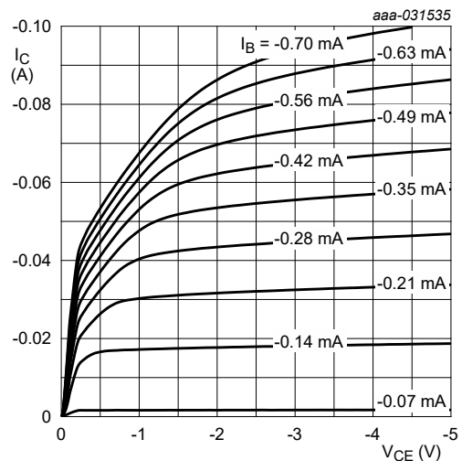
Fig. 10. NHUMD3-Q, TR2 (PNP): Collector current as a function of collector-emitter voltage; typical values
