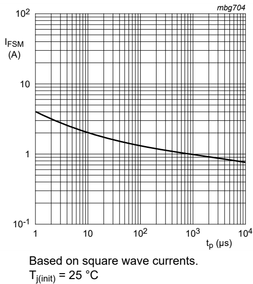
Fig. 6. Non-repetitive peak forward current as a function of pulse duration; typical values
