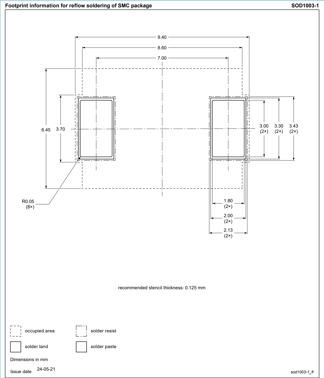
Fig. 14. Reflow soldering footprint for SMC (SOD1003-1)
