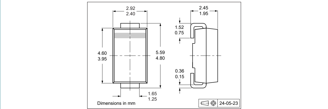
Fig. 13. Package outline SMA (SOD1001-1)
