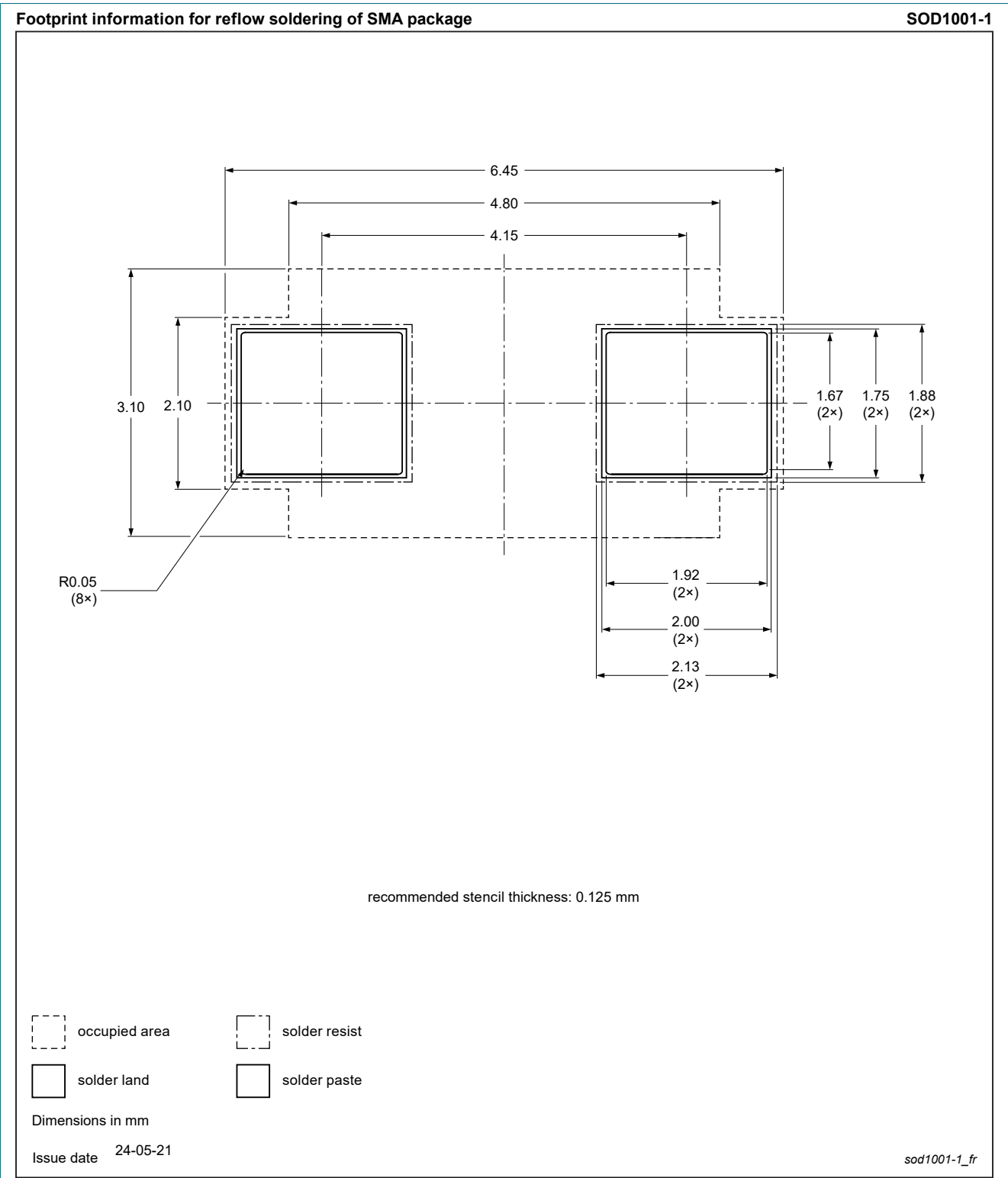
Fig. 13. Reflow soldering footprint for SMA (SOD1001-1)
