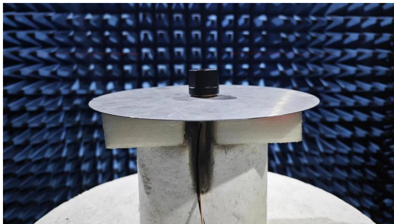
Radiation element is test on D300mm ground plane
