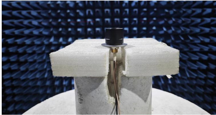
Radiation element is test on D60mm ground plane (D60mm flat washer is standard part in the packing)
