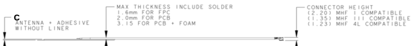
Side View
