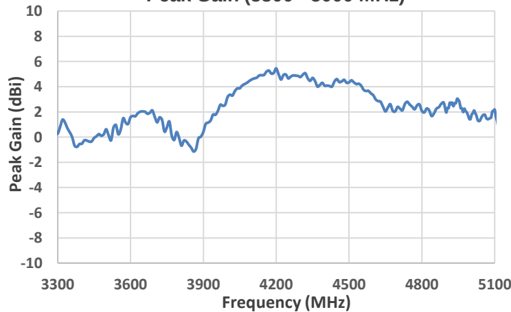
Peak Gain (3300 - 5000 MHz)
