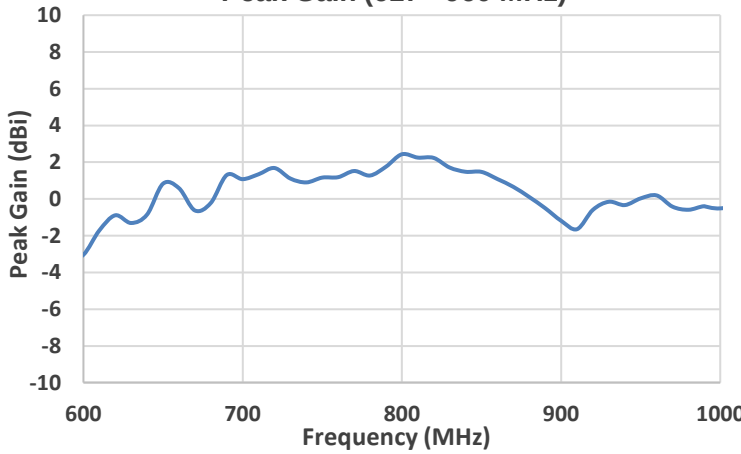
Peak Gain (617 - 960 MHz)
