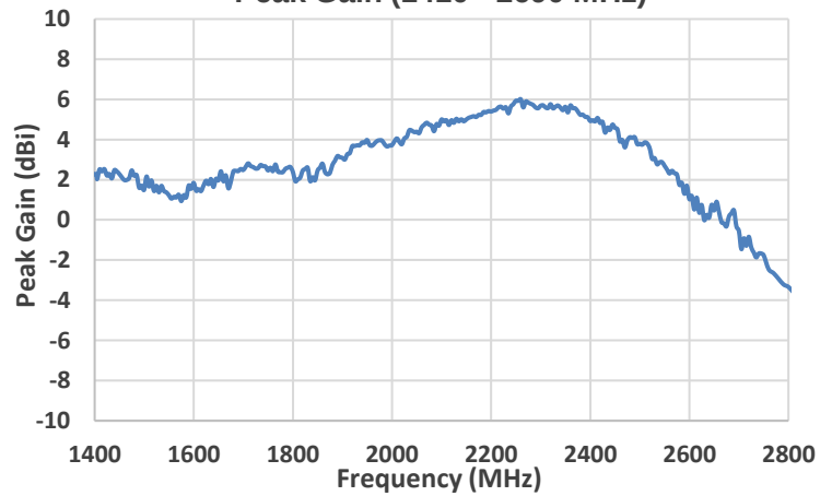
Peak Gain (1410 - 2690 MHz)
