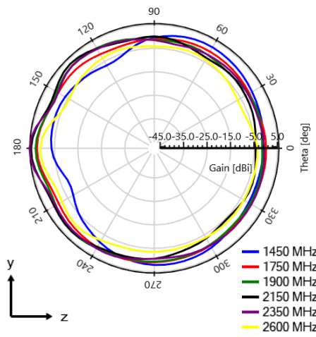
Measured (1450 - 2600 MHz)
