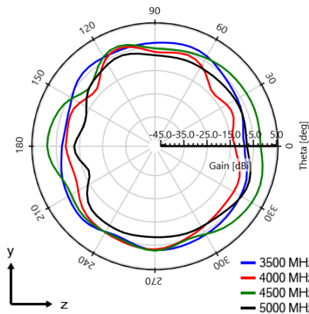
Measured (3300 – 5000 MHz)
