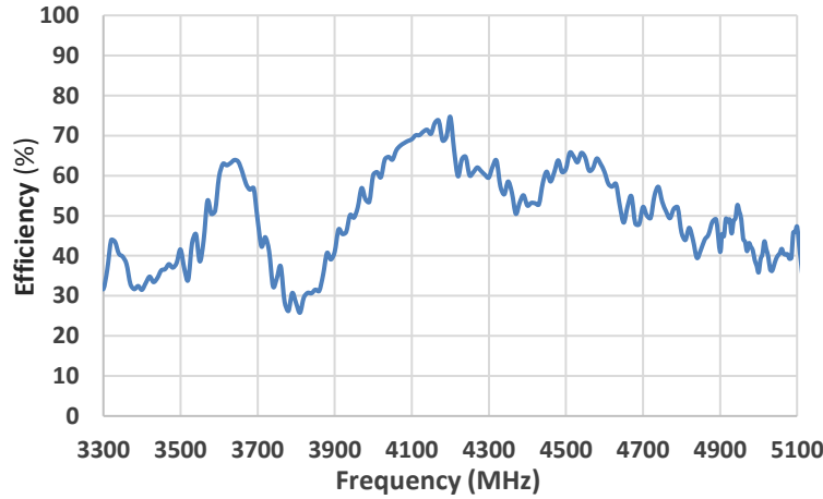
Efficiency (3300 - 5000 MHz)
