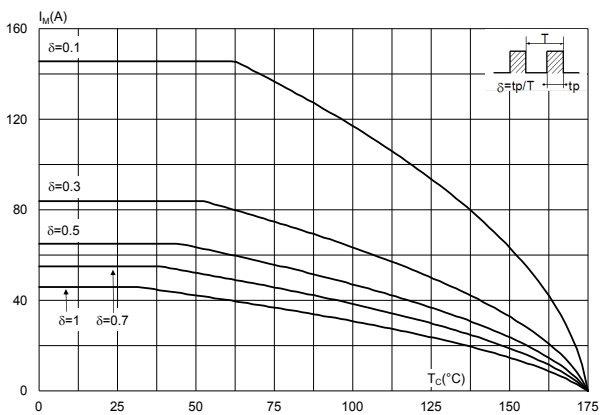
Figure 4. Peak forward current versus case temperature ( f_{\text{sw}} > 10 \text{ kHz} )
