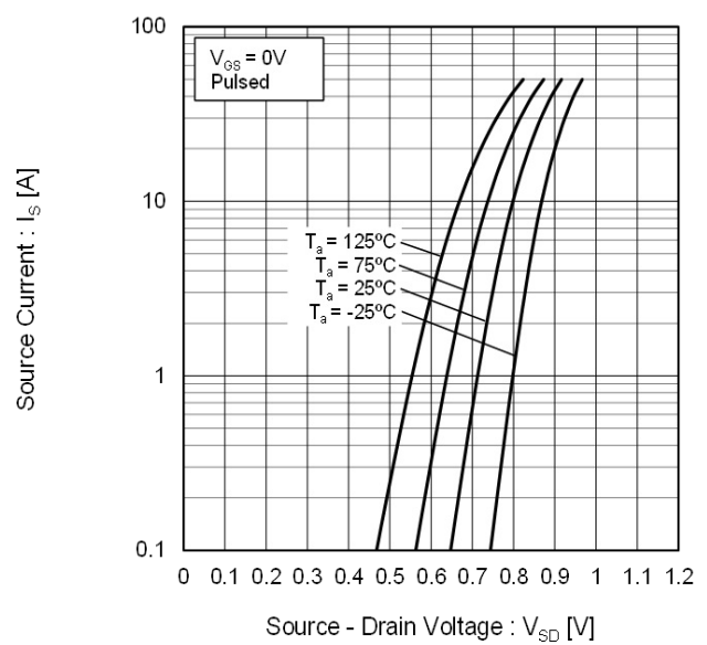
Fig.20 Source Current vs. Source Drain Voltage Source Current vs. Source Drain Voltage
