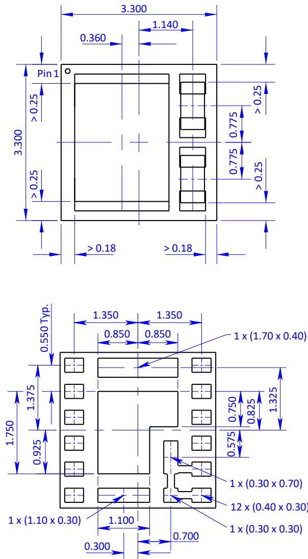
Figure 19 Dimensioned drawings
