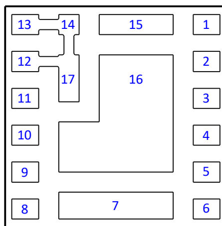
Figure 2 Pin layout (bottom view)
