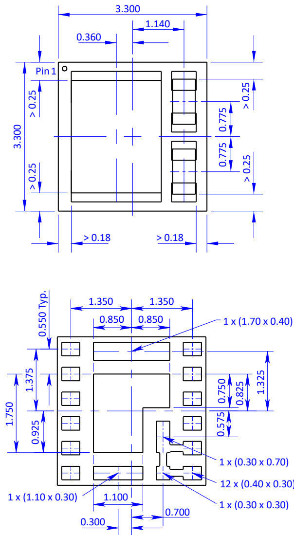
Figure 19 Dimensioned drawings
