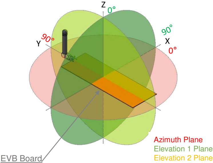
Elevation 1(XZ)
