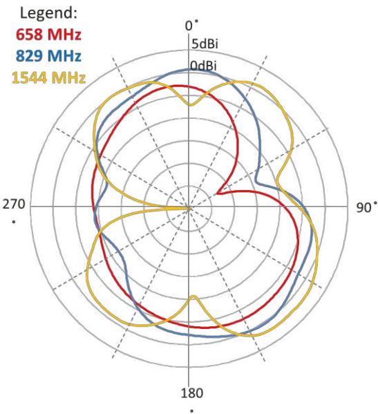
Elevation 2(YZ)
