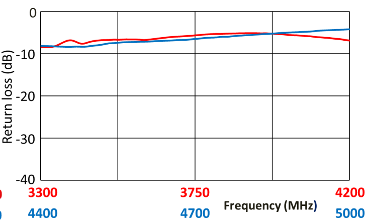
Return Loss
