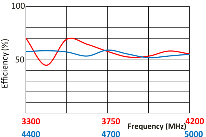
Efficiency
