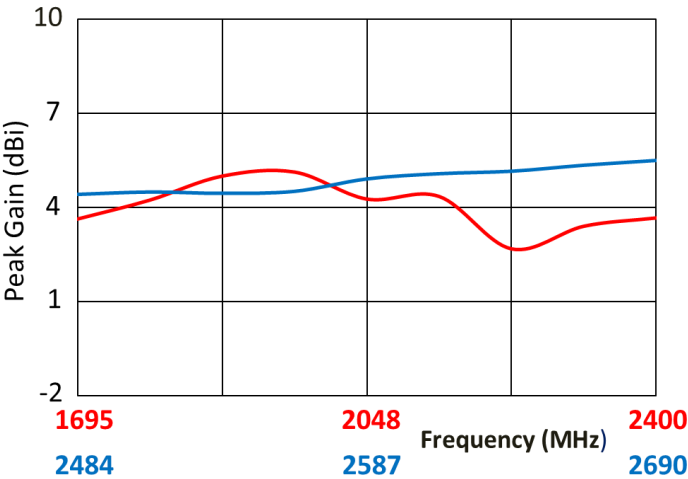
Peak Gain
