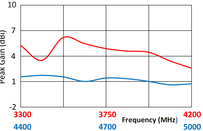
Peak Gain
