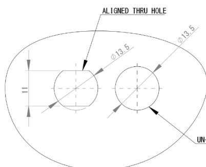
Mounting Hole Recommendation
