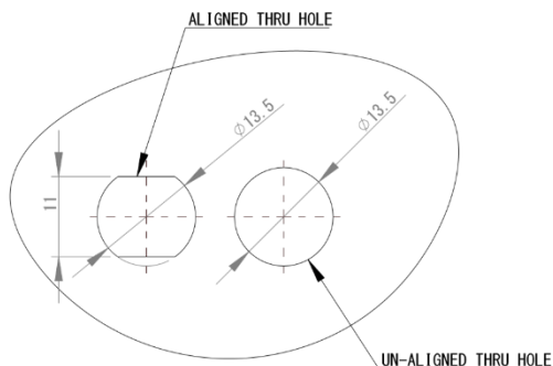
Mounting Hole Recommendation
