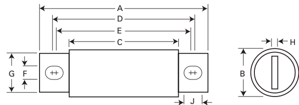
Dimensions — in
