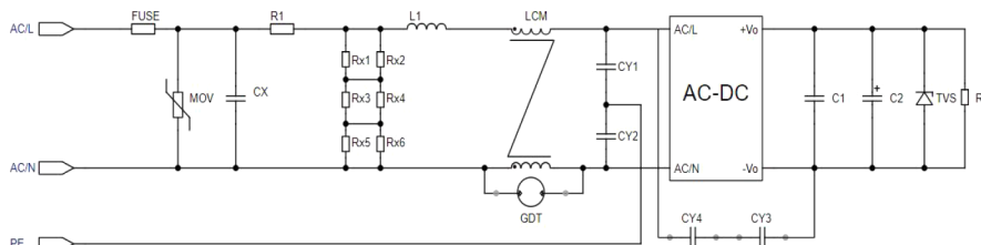
Figure 3 : category I device recommendation circuit
