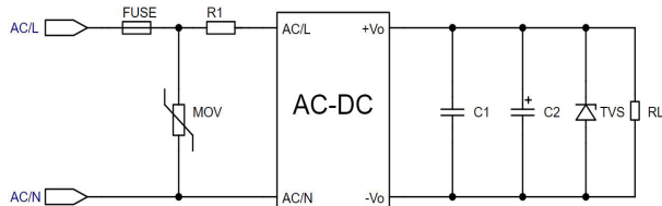
Figure 2:EMC Recommended circuits for higher requirements
