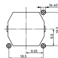
Soldering pads to Case AS21, AS35
