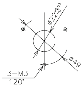
Servo Mount
