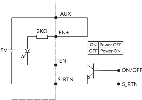
(B) Using external transistor
