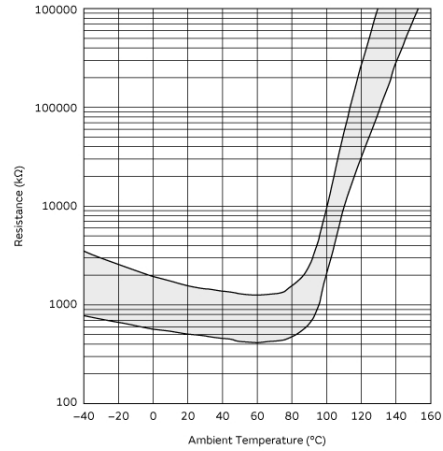
Resistance-Temperature Characteristics Range (Reference)
