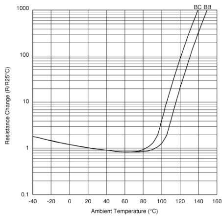
Resistance-Temperature Characteristics
