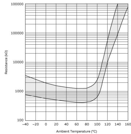
Resistance-Temperature Characteristics Range (Reference)
