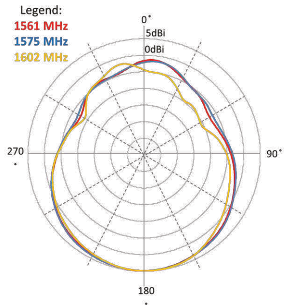
Elevation 2 (YZ)
