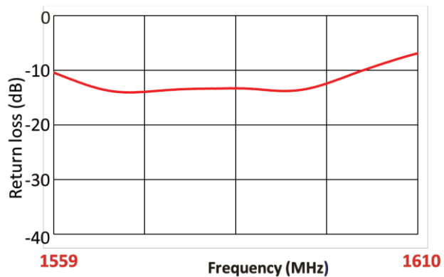
Return Loss
