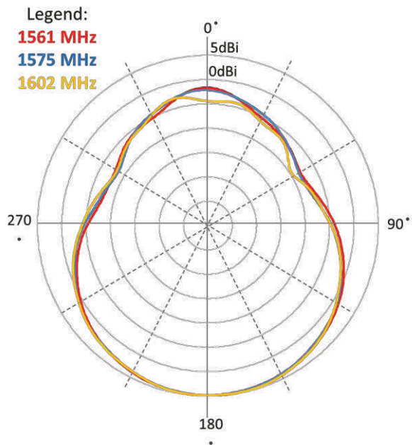
Elevation 1(XZ)
