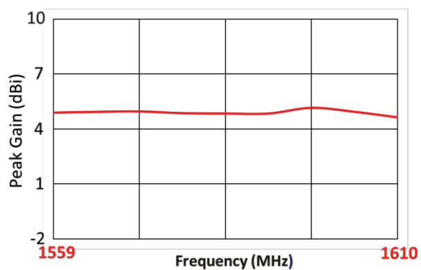
Peak Gain
