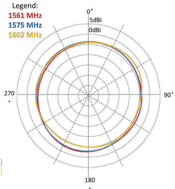
Elevation 2 (YZ)
