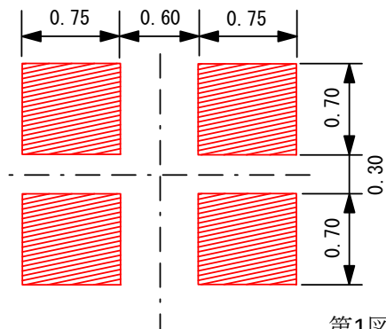
Figure 1. Dimensions
