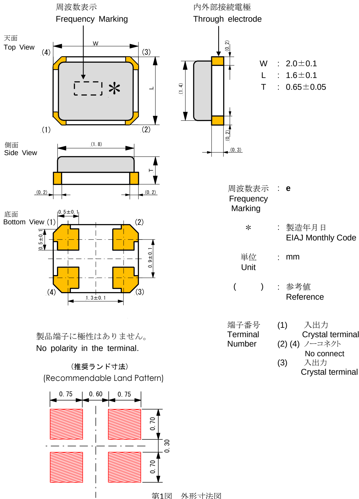
Figure 1. Dimensions
