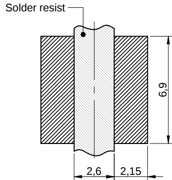
no vias and traces in restricted area Scale - 4:1
