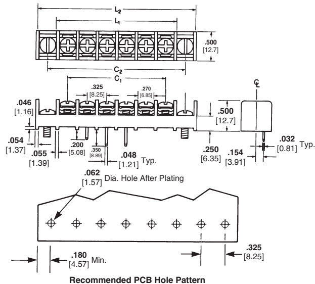
Recommended PCB Hole Pattern
