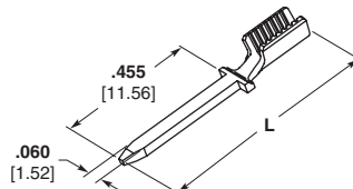
A - .060 Series Wire Crimp Tab
