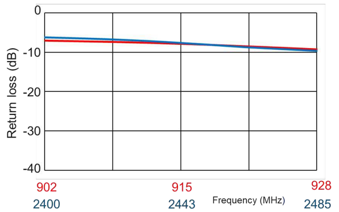
Return Loss
