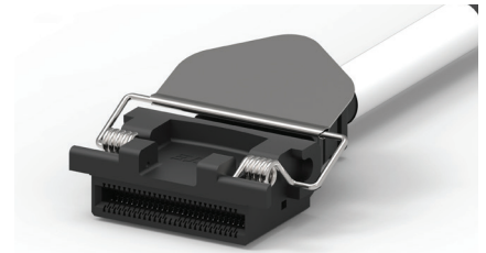
Linear Card Edge (LEC) Receptacle - mates to Intel processors
