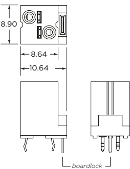
2 position screwless wire connector4
