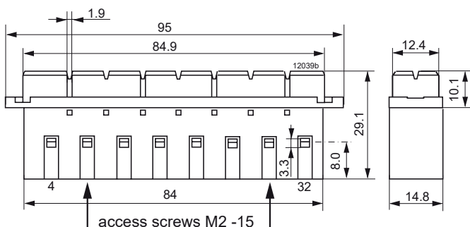
Fig. 8 HZZ00107-G: screw terminals, max. torque 26.6 Ncm, material LPC E130i HZZ00106-G: faston terminals 6.3 × 0.8 mm (similar dimensions, but not shown). The orientation of the faston terminals can be horizontal or vertical, depending on supplier.
