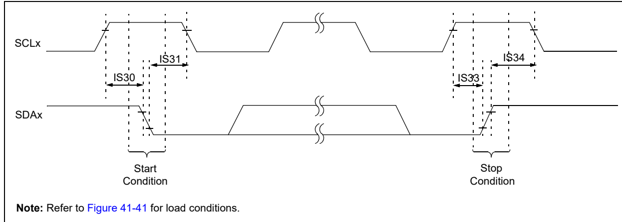
FIGURE 41-57: I2Cx BUS START/STOP BITS TIMING CHARACTERISTICS (CLIENT MODE)
