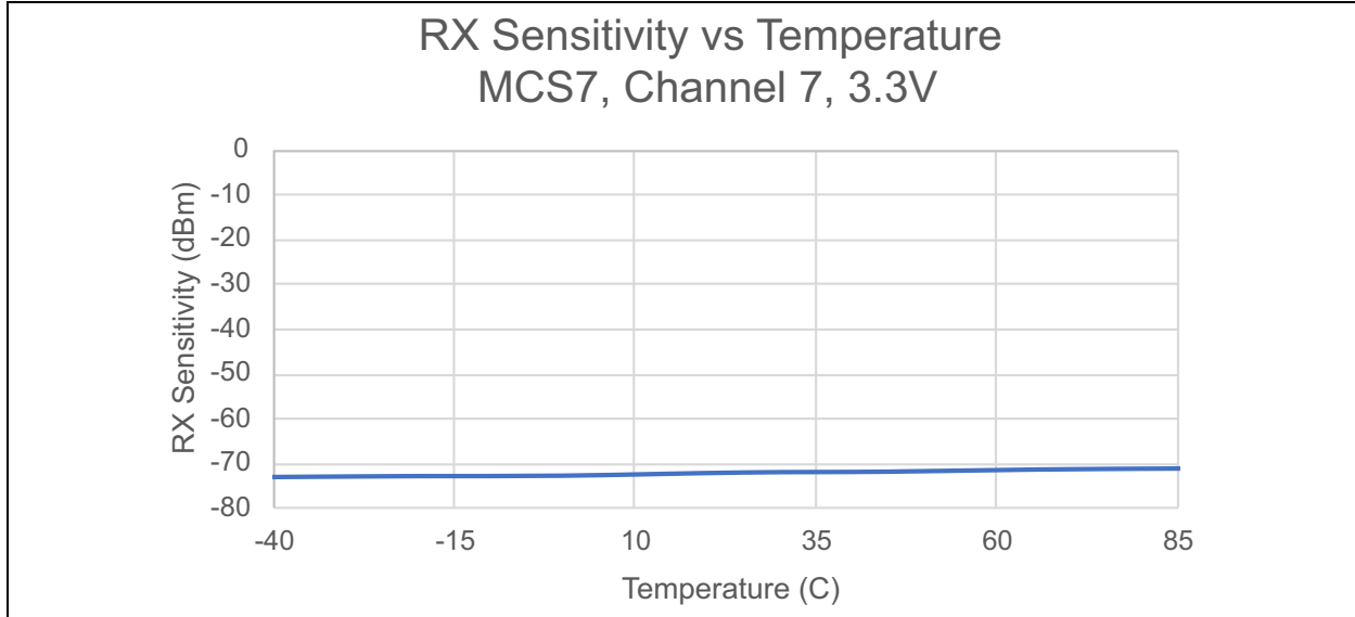
FIGURE 41-100: RX SENSITIVITY VS TEMPERATURE
