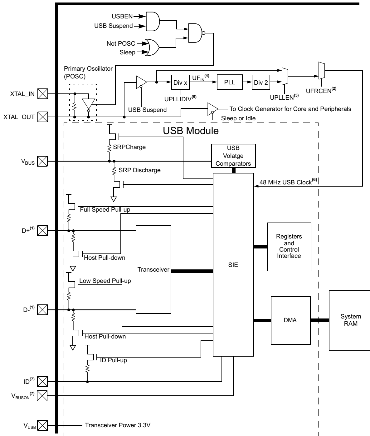
FIGURE 12-1: PIC32MZ W1 Family USB INTERFACE DIAGRAM
