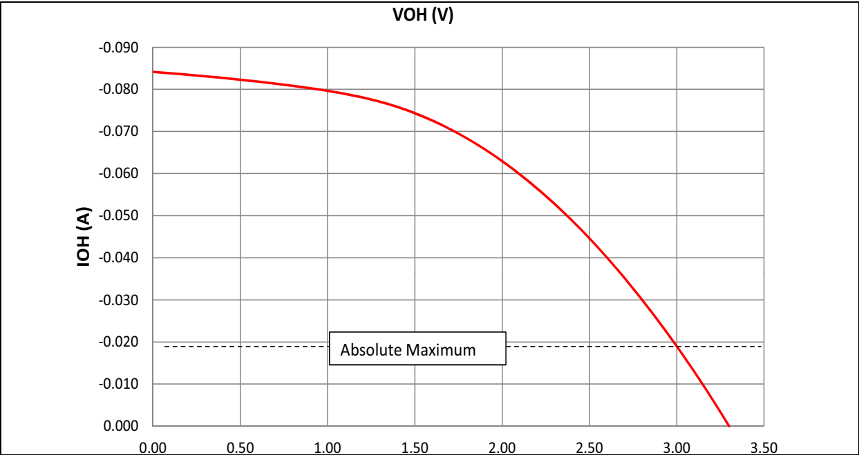
FIGURE 41-25: V_{OH} – 8x DRIVER PINS
