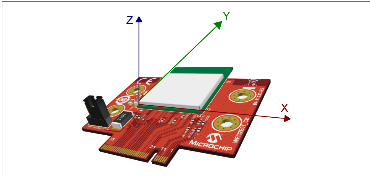
FIGURE 3-19: MODULE ORIENTATION FOR RADIATION PATTERN MEASUREMENT
