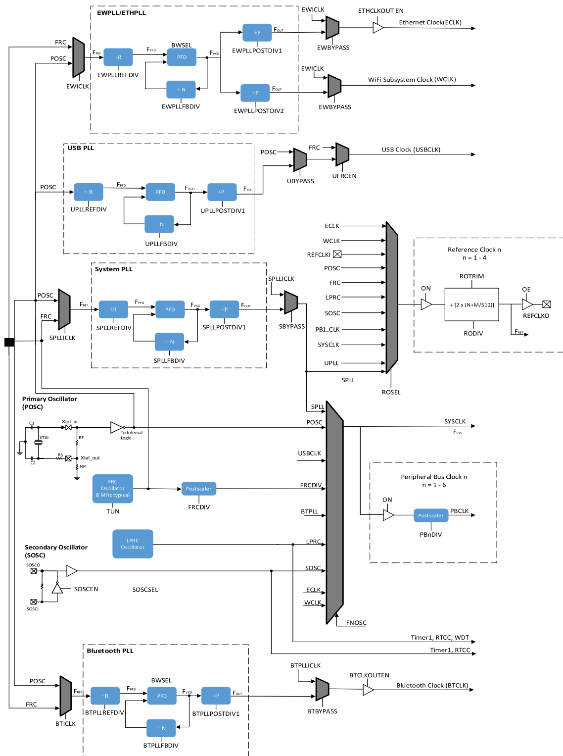
FIGURE 11-1: PIC32MZ W1 FAMILY OSCILLATOR DIAGRAM
