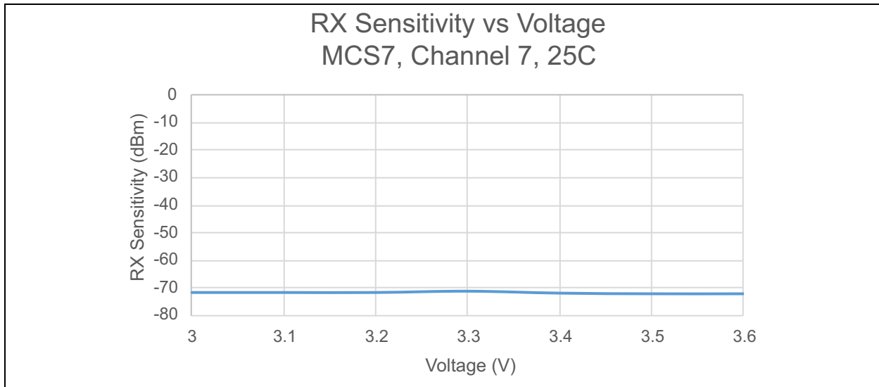
FIGURE 41-36: RX SENSITIVITY VS VOLTAGE
