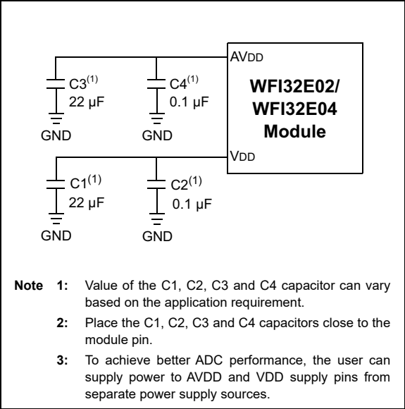
FIGURE 3-8: WFI32E02/WFI32E04 RECOMMENDED MODULE POWER SUPPLY CONNECTIONS
