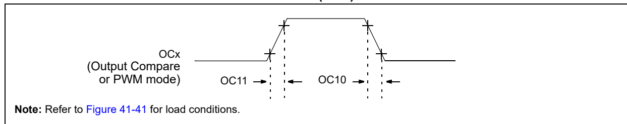
FIGURE 41-48: OUTPUT COMPARE MODULE (OCx) TIMING CHARACTERISTICS
