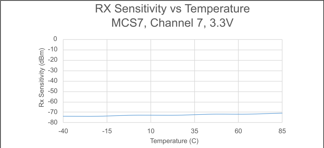
FIGURE 41-87: RX SENSITIVITY VS TEMPERATURE
