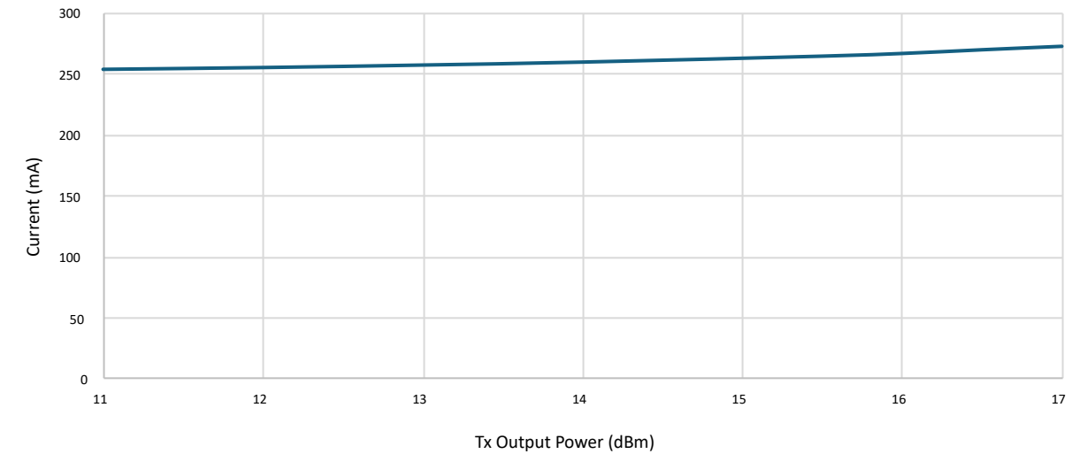
Figure 3-4. Transmit Current vs Transmit Output Power, MCS7, Channel 7, 3.3V, 25°C
