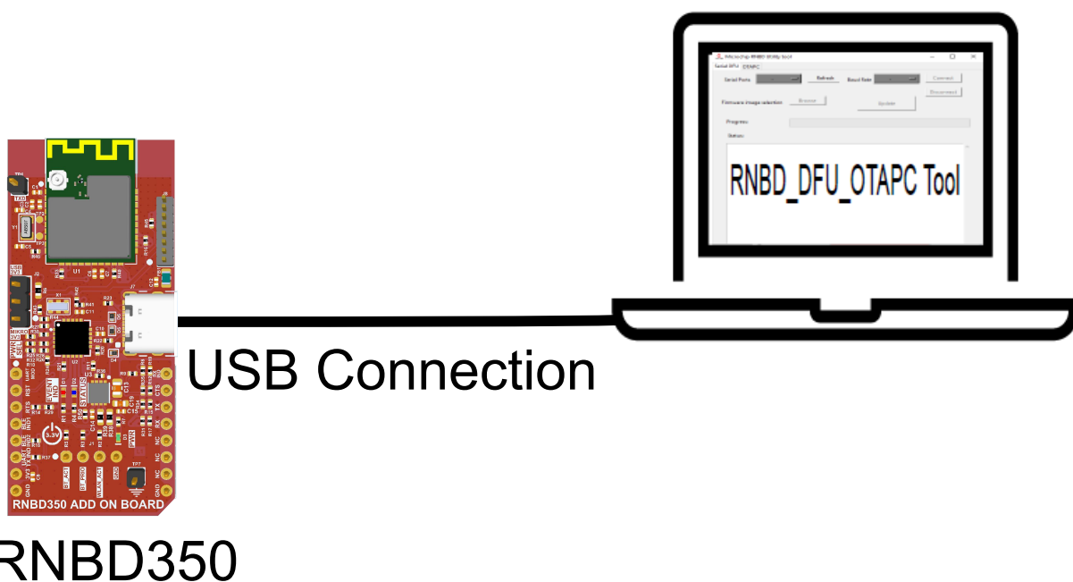
Figure 5-11. Serial DFU Block Diagram
