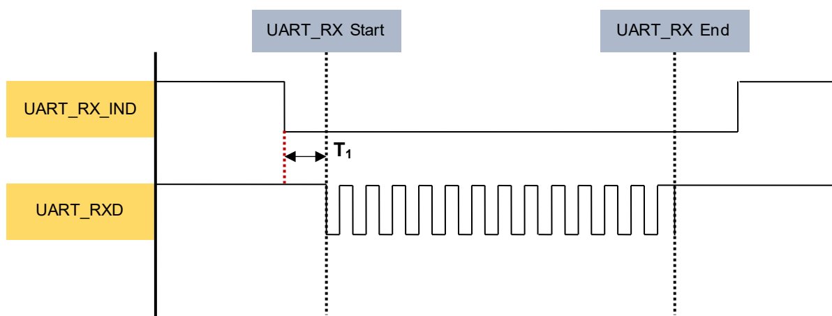
Figure 5-3. Wake Up RNBD350 from DSADV Timing Diagram
