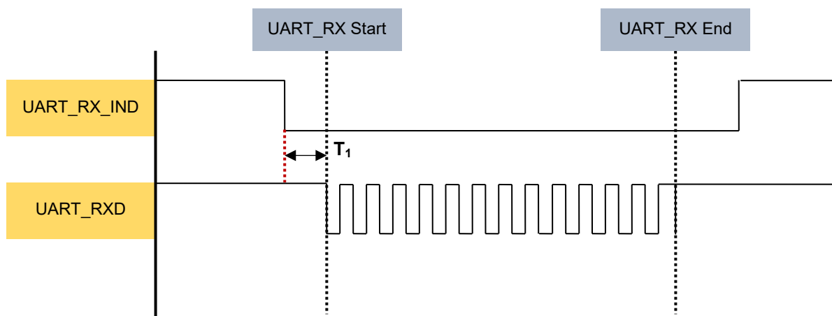
Figure 5-2. Wake Up RNBD350 from Sleep Mode Timing Diagram
