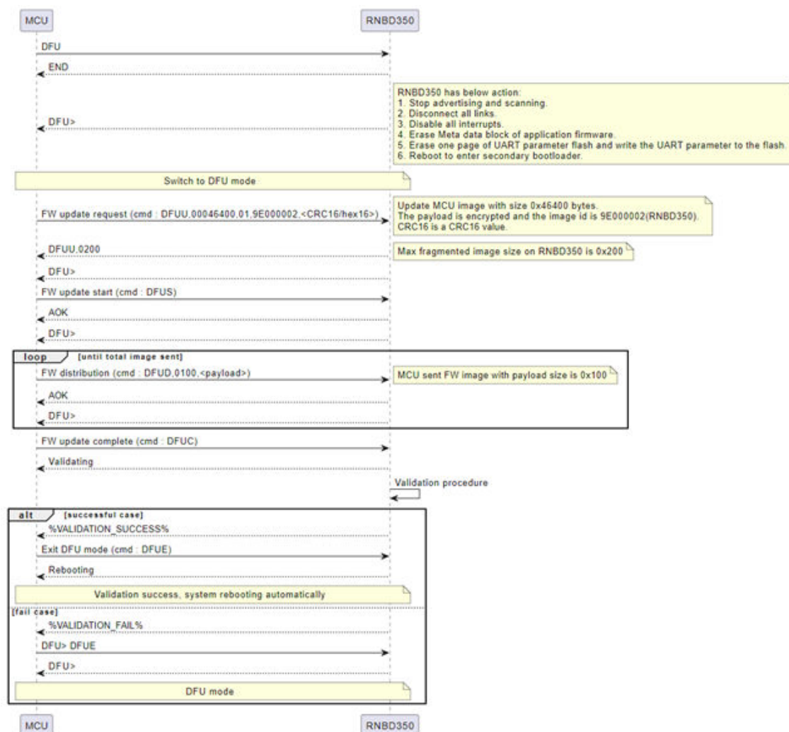
Figure 5-13. MSC for DFU
