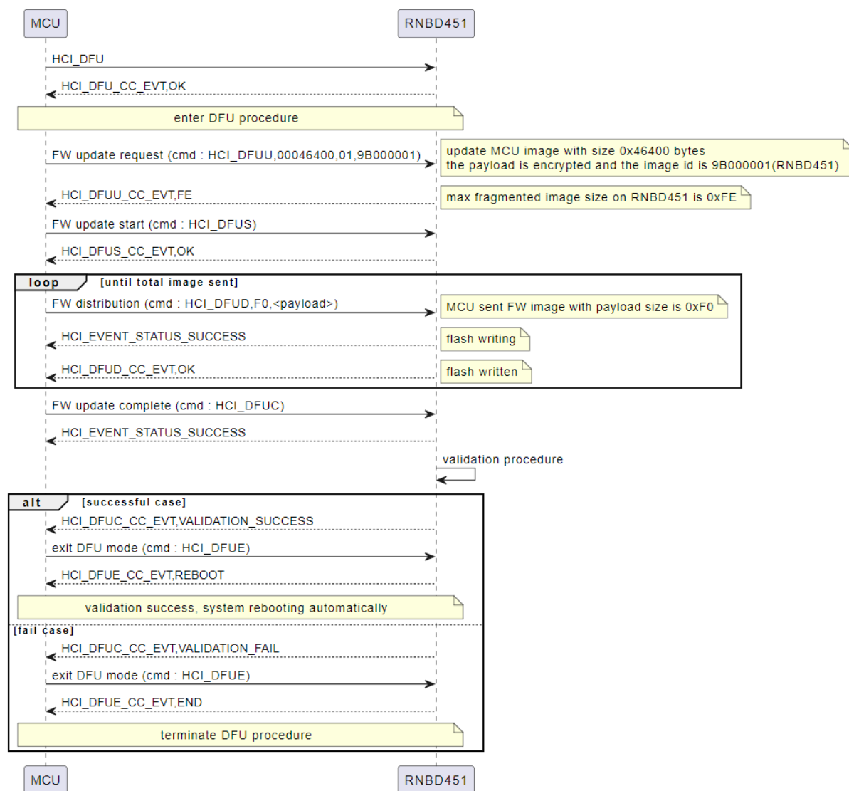
Figure 6-1. HCI DFU Procedure
