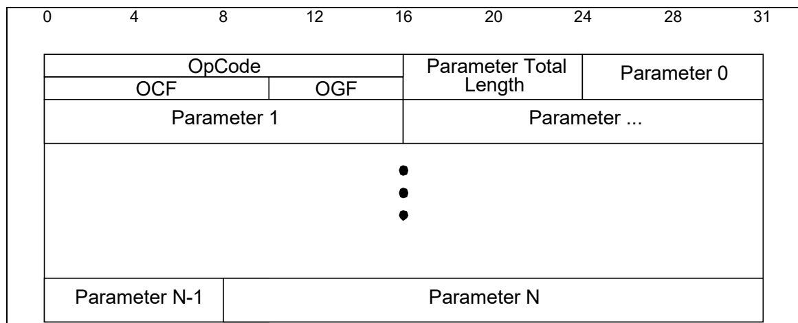
Figure 5-5. HCI Command Format
