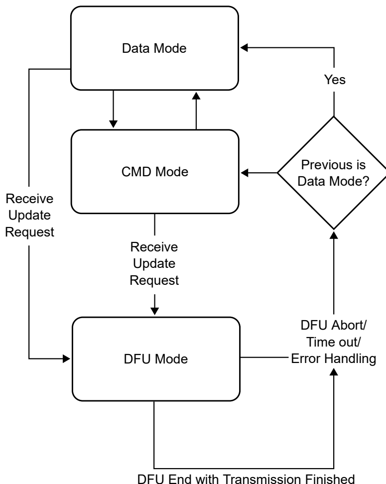
Figure 5-16. Host OTA through RNBD350 Transition Diagram
