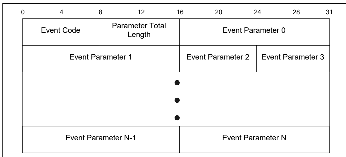
Figure 5-6. HCI Event Format
