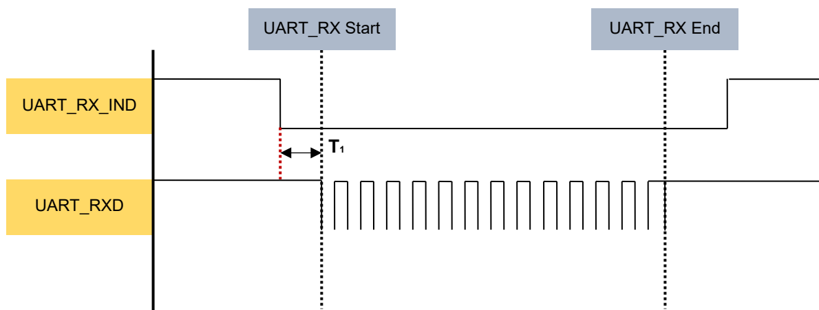
Figure 5-1. Wake-Up the RNBD350 Module from XDS Timing Diagram
