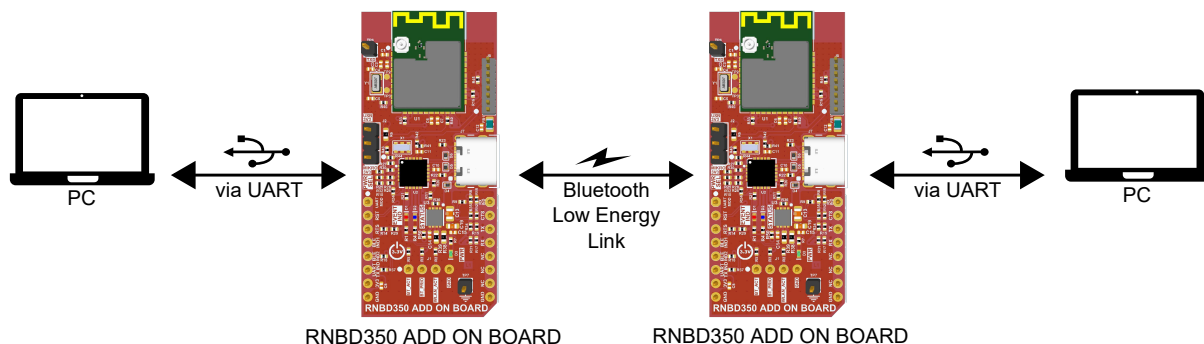
Figure 7-34. Module to Module Connection
