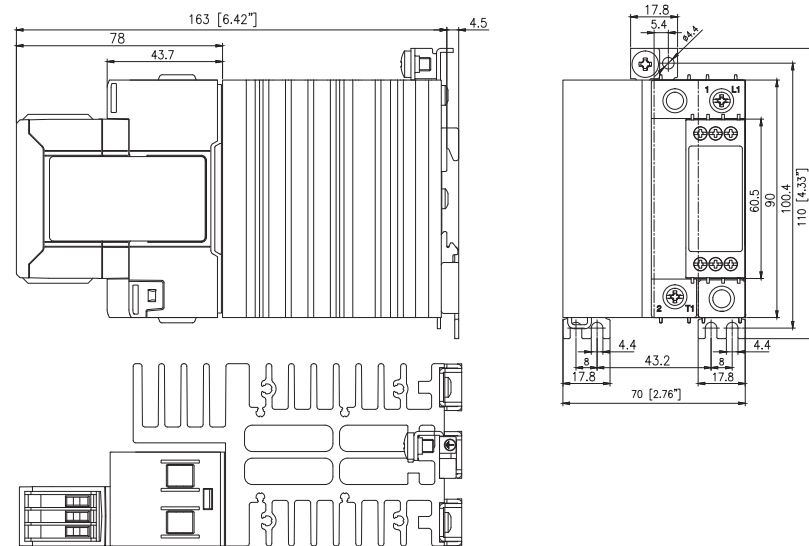
RGC1S60D90GGEP (fan to be supplied externally - no terminations provided on the RG module)
