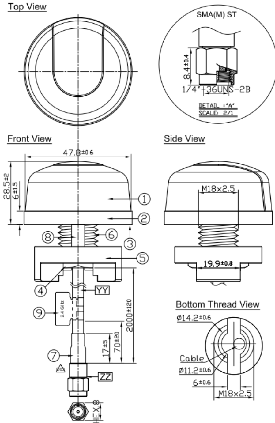
Figure 15. Technical Drawing
