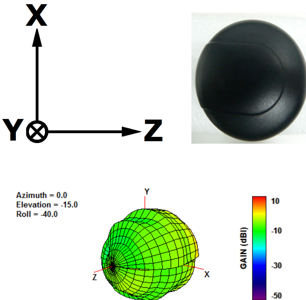
Figure 13. 3D Radiation Pattern at 2450 MHz of the WS.02 Antenna with standard 2 meter cable
