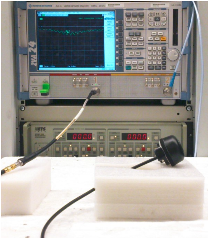
Figure 1. Return loss measurements.
