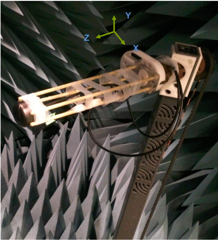
Figure 2. Peak gain, efficiency and radiation pattern measurements
