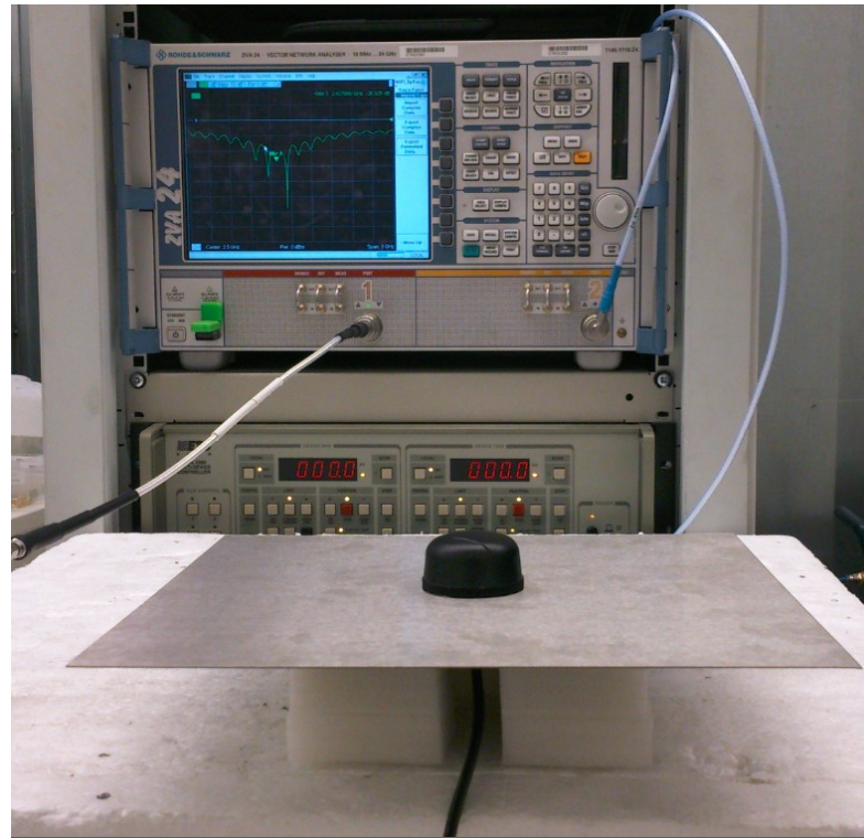
Figure 1. Return loss measurements.
